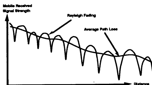
Figure 3. Mobile Received Signal Strength in Log-Normal Shadowing and Rayleigh Fading
