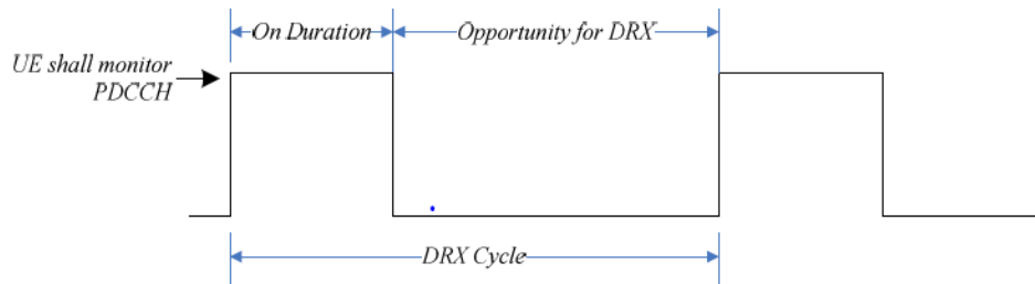
Figure 3.1-1: DRX Cycle
