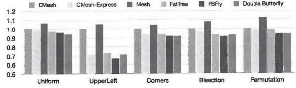
Fig. 13. Normalized runtime for additional topologies where 25% of the total traffic consists of memory references, which are uniformly distributed.
