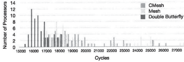
Fig. 11. Distribution of completion times with UpperLeft workload.
