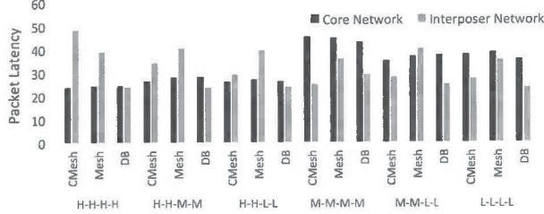
Fig. 12. Latency comparison using multi-programmed SynFull workloads.
