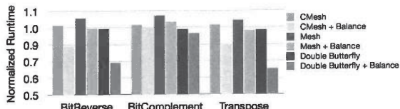
Fig. 15. Load balancing across layers with 25% of total traffic consisting of memory references and non-uniformly distributed CPU traffic.
