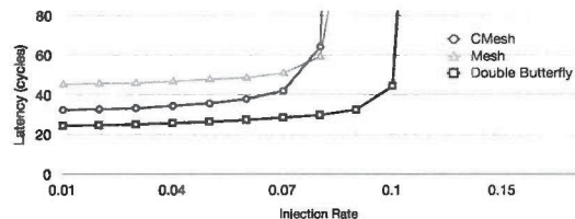
Fig. 8. Load-latency curves with uniformly-distributed memory references.
