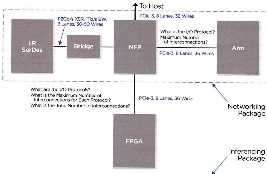
Figure 20. Networking and inferencing package on demo system
