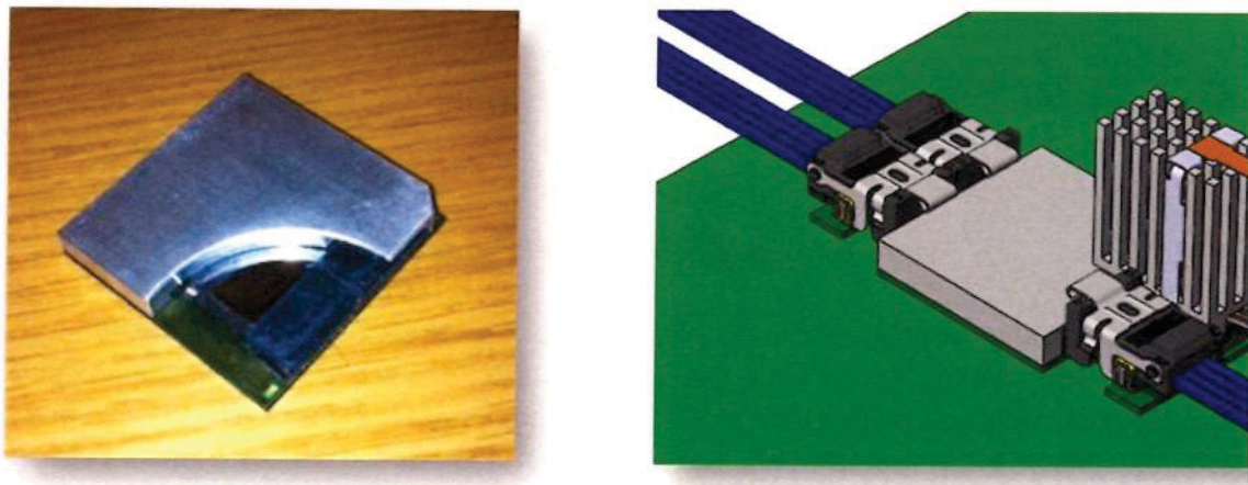
Figure 14: Two Firefly connectors embedded in a 45mm square package
