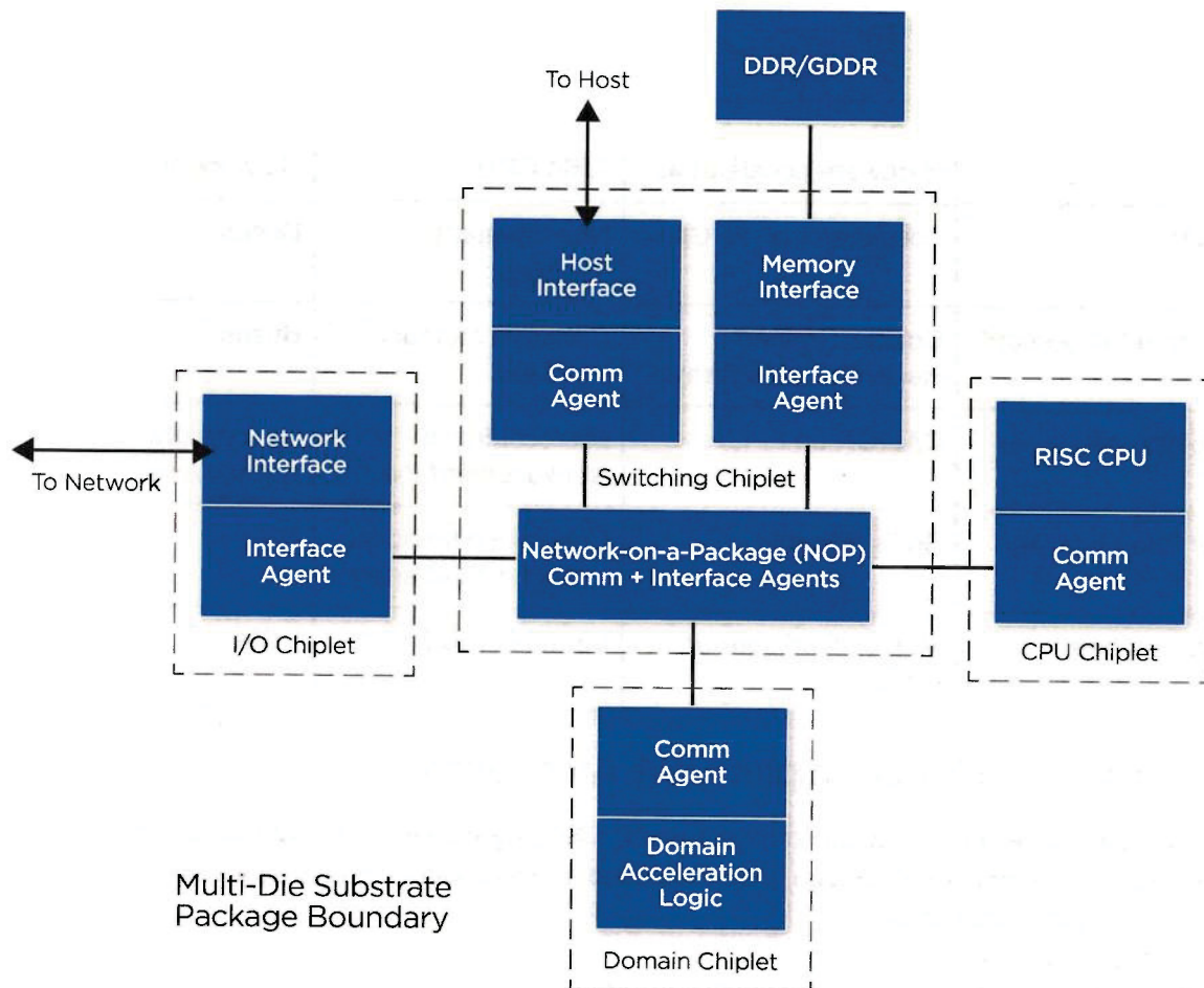
Figure 18: Reference multi-die architecture
