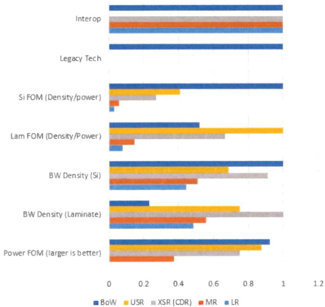
Figure 6: Comparing die-to-die protocols
