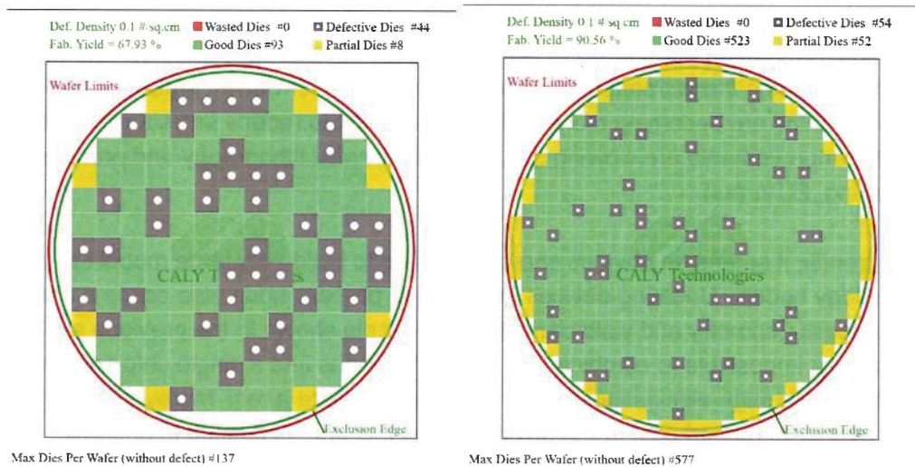
Figure 3: Die size impact on yield
