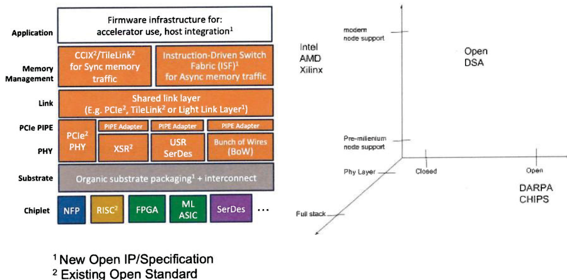
Figure 1: The ODSA protocol stack and focus area
