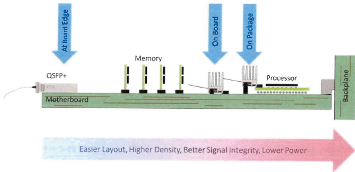
Figure 13: Connector positioning for fiber to the package
