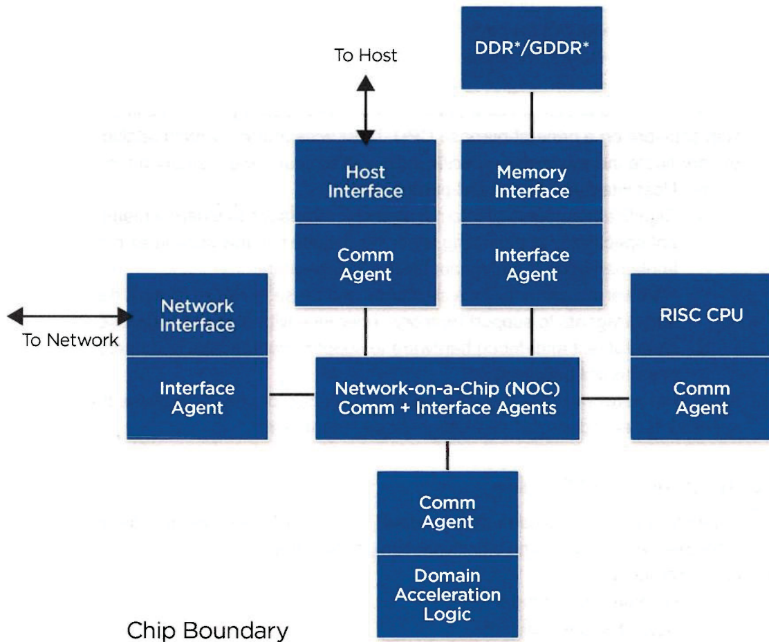
Figure 17: Reference monolithic domain-specific accelerator architecture
