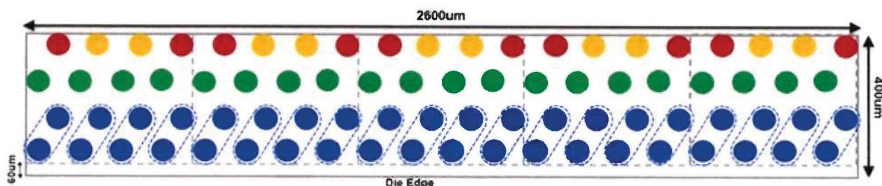
Figure 10: AQLink-500G bump map
