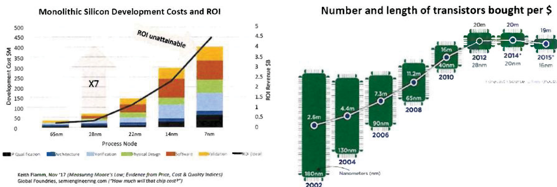
Figure 2: ASIC development costs and transistor cost efficiency
