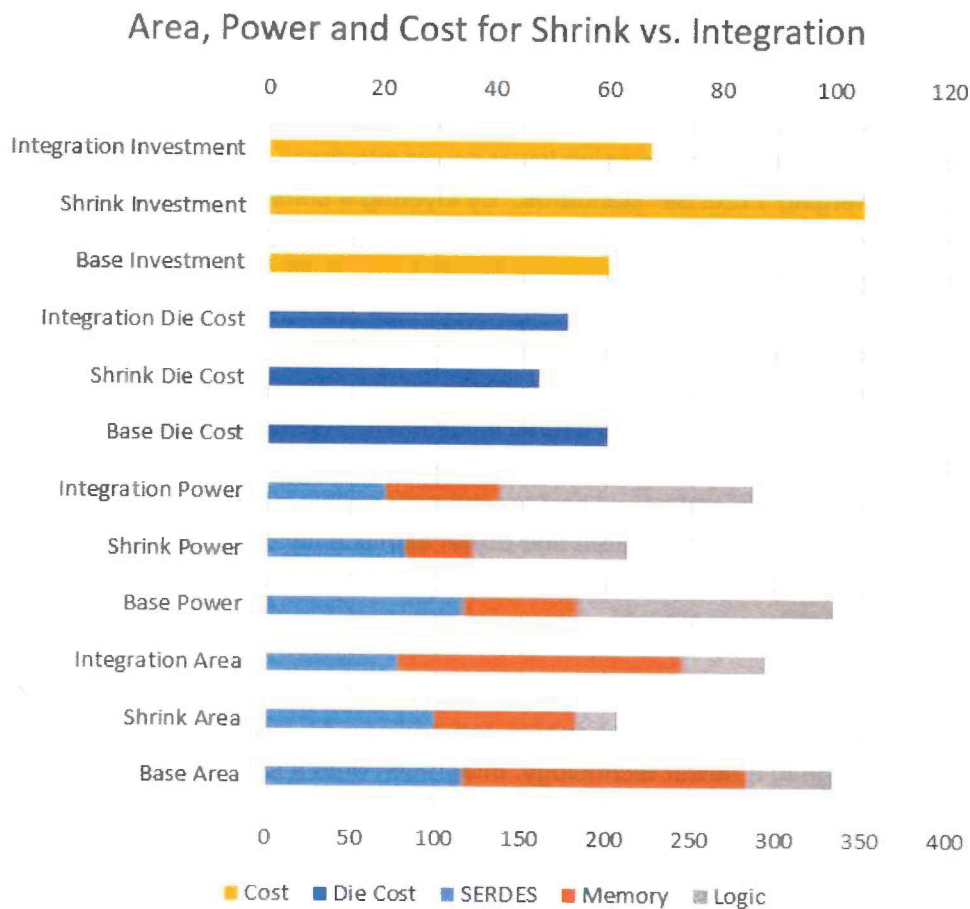
Figure 5: Comparing(multi-chip) integration with a process node shrink
