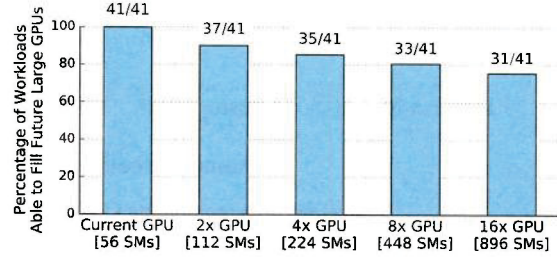
Figure 2: Percentage of workloads that are able to fill future larger GPUs (average number of concurrent thread blocks exceeds number of SMs in the system).
