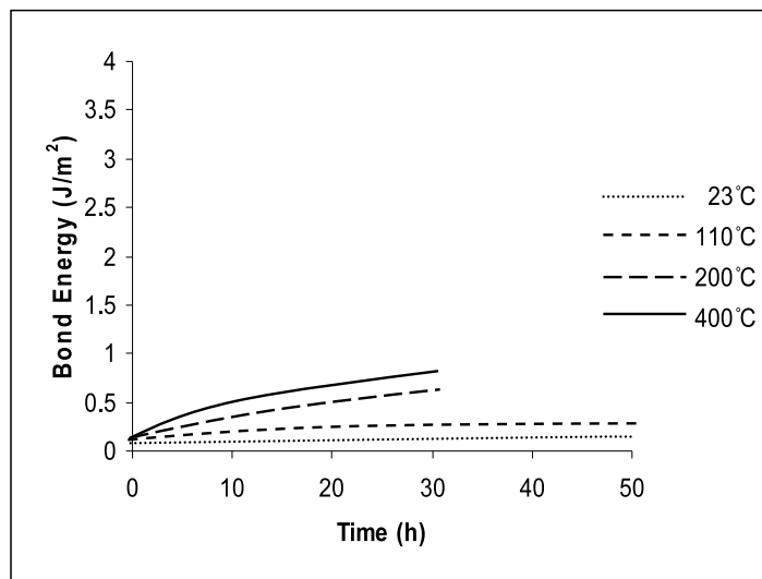
Fig. 1. Typical bonding energy vs time for conventional direct wafer bonding at postbond temperatures of 23°C, 110°C, 200°C, and 400°C of 100 mm PECVD coated silicon wafers.
