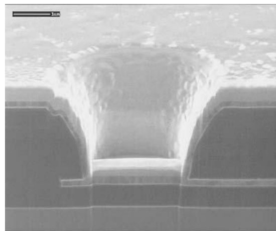
Fig. 5. SEM cross section of FIB cut of ROIC wafer ZiROC bonded to detector wafer with two micron via and metal interconnection between ROIC and detector wafers.
