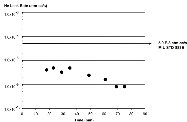
Fig. 3. Helium partial pressure vs posthelium pressure time for ZiROC bonded silicon cavity to silicon wafer.
