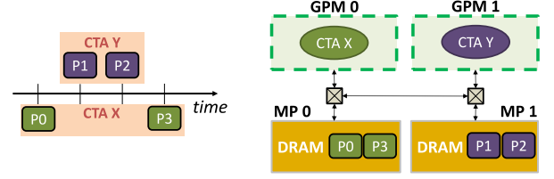
Figure 11: First Touch page mapping policy: (a) Access order. (b) Proposed page mapping policy
