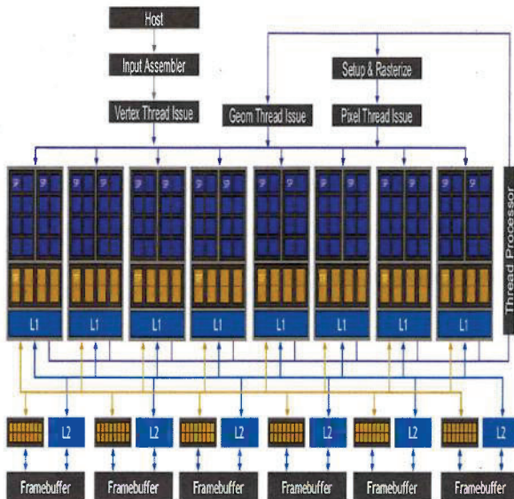
Illustration 7: GeForce 8 Architecture
