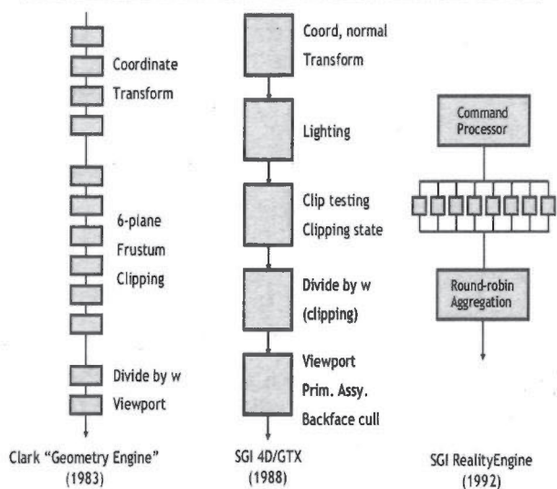
Illustration 2: Early trends in pipeline parallelism
