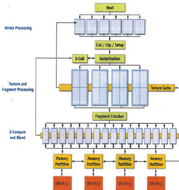
Illustration 5: GeForce 6 Architecture
