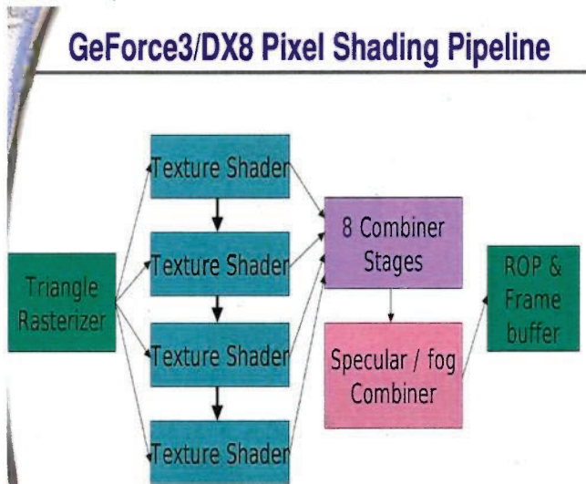
Illustration 4: GeForce 3 Architecture
