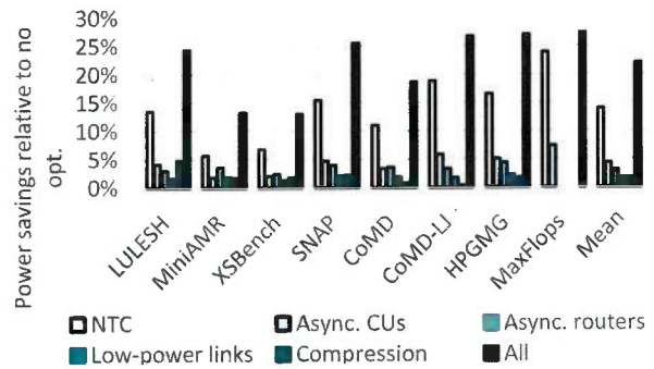
Figure 12. Power savings from optimizations
