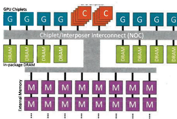
Figure 3. Block diagram of the ENA memory system
