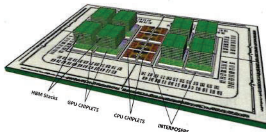
Figure 2. Exascale Heterogeneous Processor (EHP)
