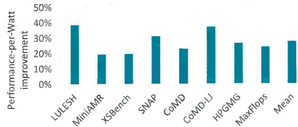
Figure 13. Energy-efficiency benefit from optimizations
