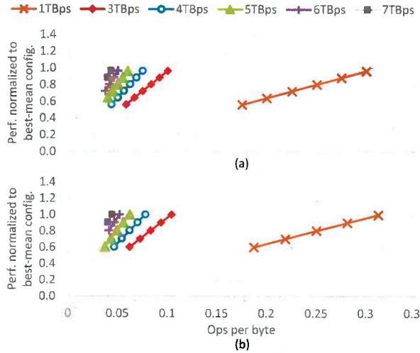
Figure 4. Performance of MaxFlops as we vary the bandwidth and (a) CU frequency or (b) CU count
