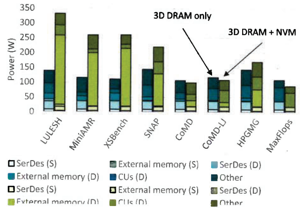
Figure 9. Impact of external-memory configurations on ENA power
