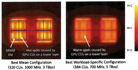
Figure 11. Heat map of the bottom-most in-package 3D-DRAM die for SNAP
