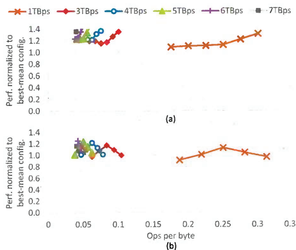
Figure 6. Performance of LULESH as we vary the bandwidth and (a) CU frequency or (b) CU count
