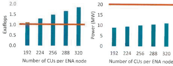
Figure 14. MaxFlops performance and power
