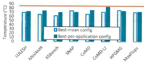
Figure 10. Peak in-package 3D-DRAM temperature
