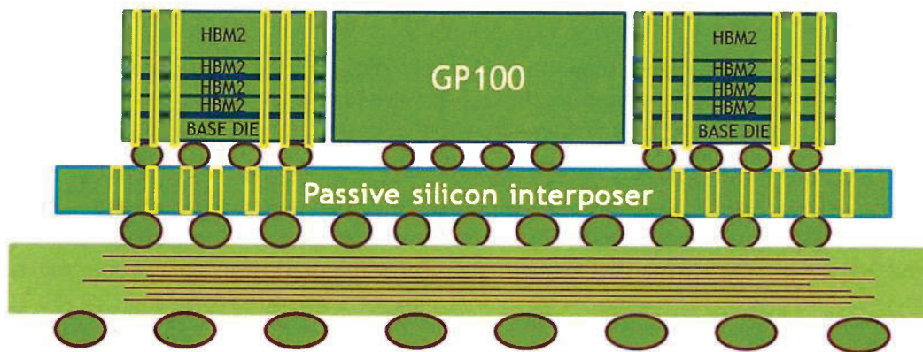
Figure 9. Cross-section illustrating GP100 adjacent HBM2 stacks
