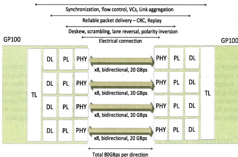
Figure 25. NVLink Layers and Links; Physical Layer (PHY), Data Link Layer (DL), Transaction Layer (TL)
