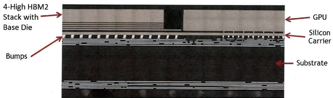
Figure 10. Cross-section Photomicrograph of a P100 HBM2 stack and GP100 GPU
