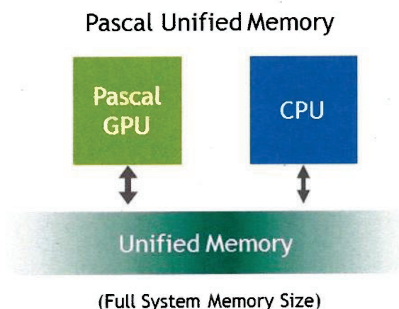
Figure 21. Pascal GP100 Unified Memory is not Limited by the Physical Size of GPU Memory.
