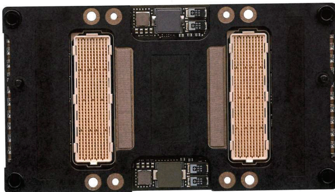
Figure 12. Tesla P100 Accelerator (Back)
