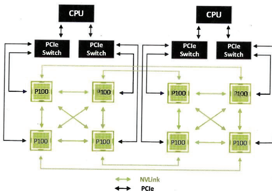
Figure 14. Eight GPU Hybrid Cube Mesh Architecture
