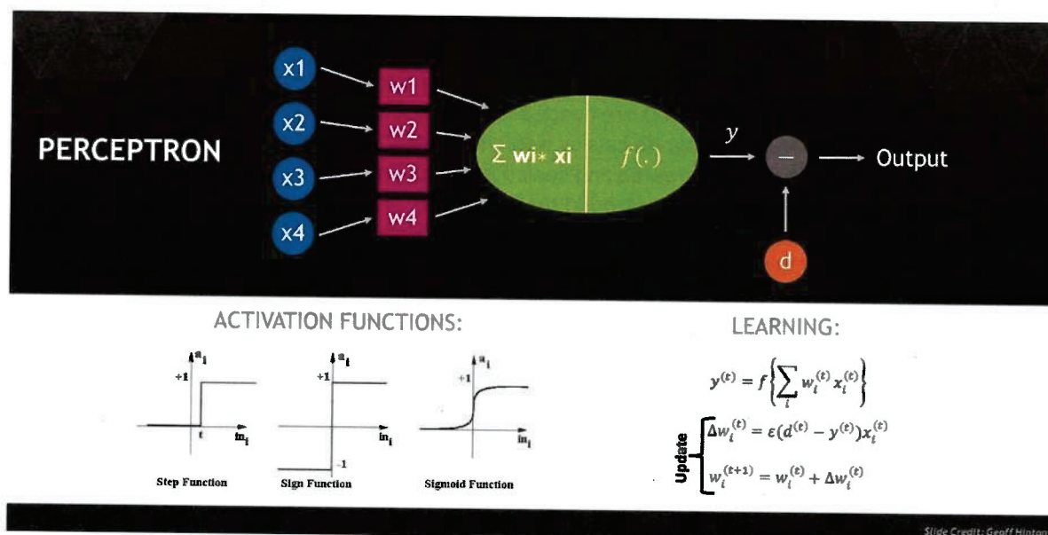
Figure 26. The Perceptron is the Simplest Model of a Neural Network
