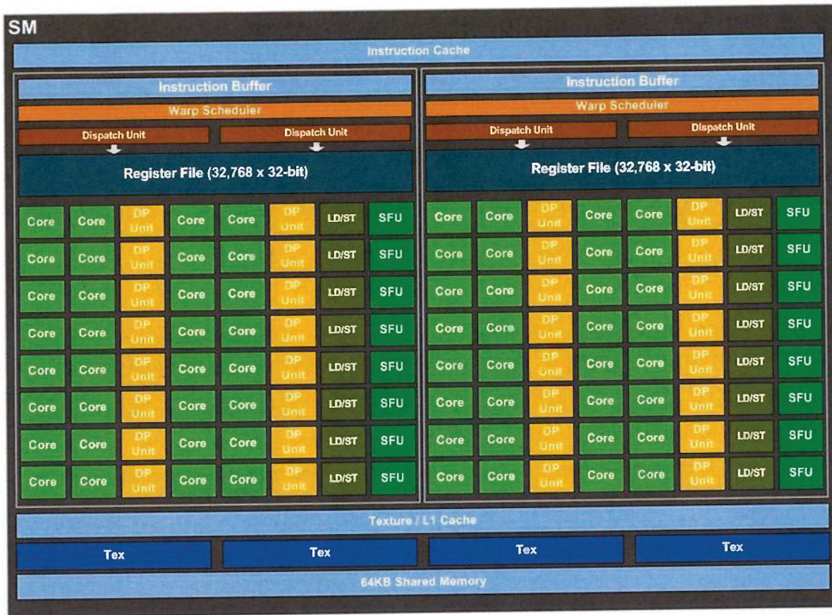
Figure 8. Pascal GP100 SM Unit
