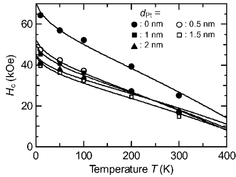
Figure 2. The coercivity H_c of the FePt nanoparticles covered with Pt [ d_{\text{Pt}} nm]/Ag [ (4 - d_{\text{Pt}}) nm] overlayers as a function of temperature. Solid curves indicate the best fittings based on the thermal fluctuation analysis.
