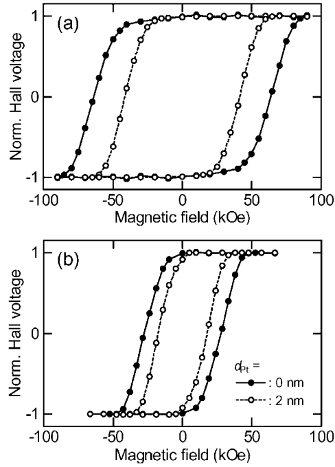
Figure 1. Normalized Hall voltage curves at (a) T = 10 K and (b) 300 K for the FePt nanoparticles covered with Pt [ d_{\text{Pt}} nm]/Ag [ (4 - d_{\text{Pt}}) nm] overlayers.
