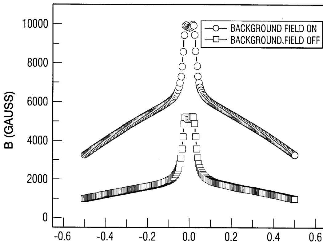
FIG. 6 DISTANCE FROM THE POLE TIP CENTER (μm)
