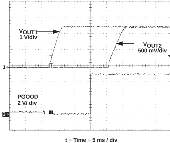
Figure 19. Offset Startup
