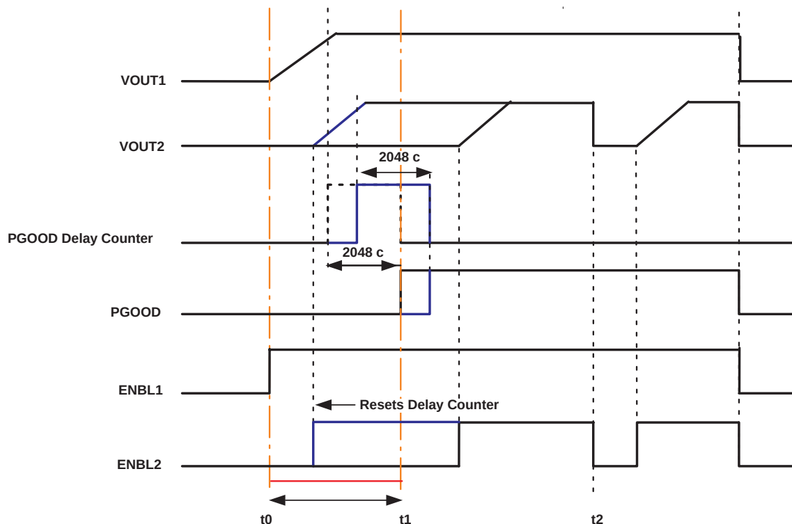
Figure 3. PowerGood Timing Diagram
