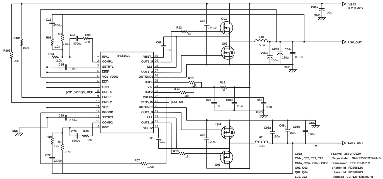
Figure 6. Typical Application Circuit: DDR(2.5V/6A + 1.25V/6A) from VBAT
