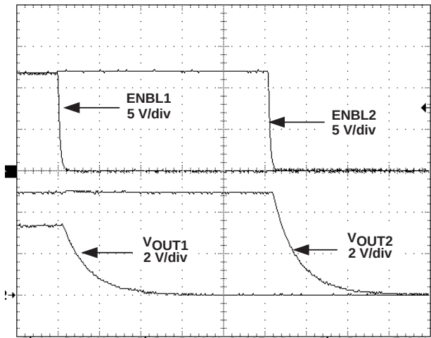
t – Time – 5 ms / div Figure 20. Soft-Stop
