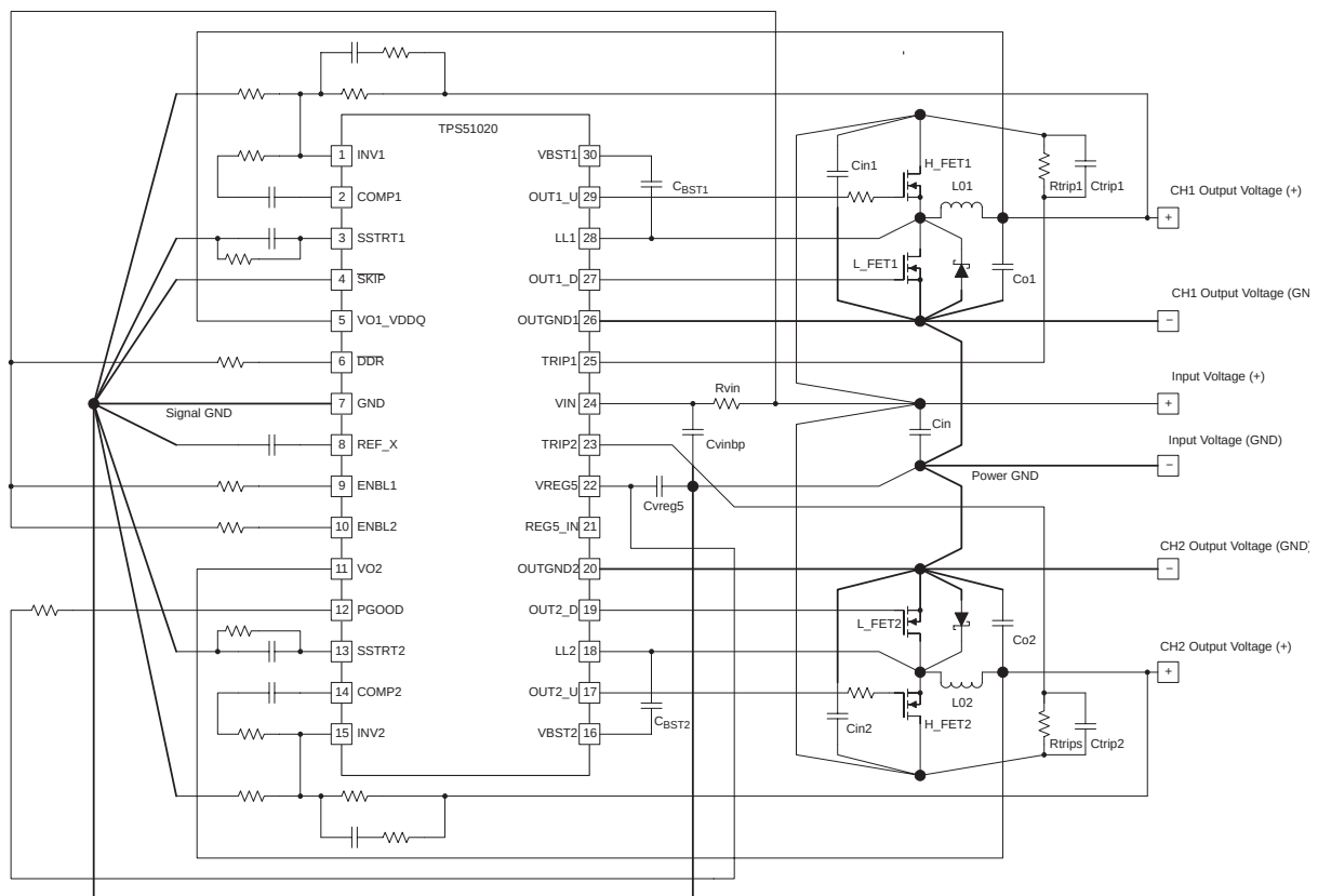
Figure 4. PCB Trace Guideline
