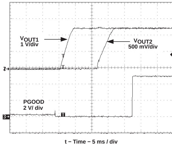
Figure 18. Simultaneous Startup
