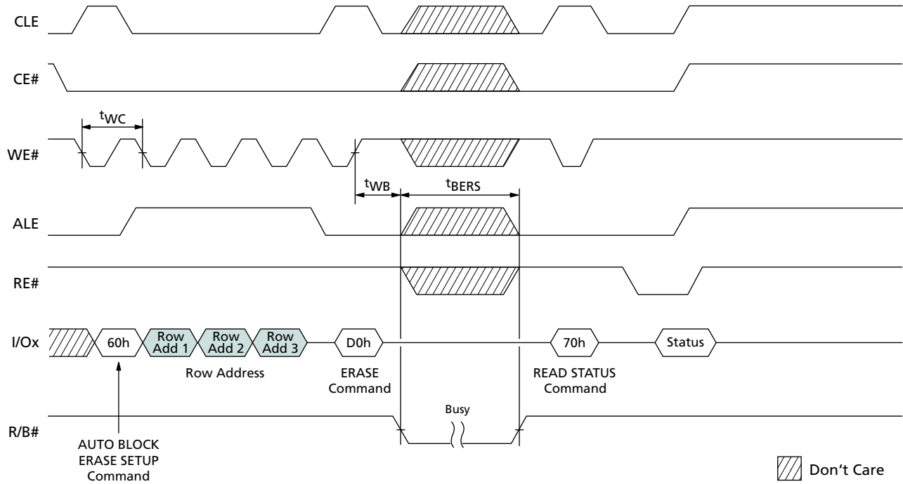
Figure 53: BLOCK ERASE Operation
