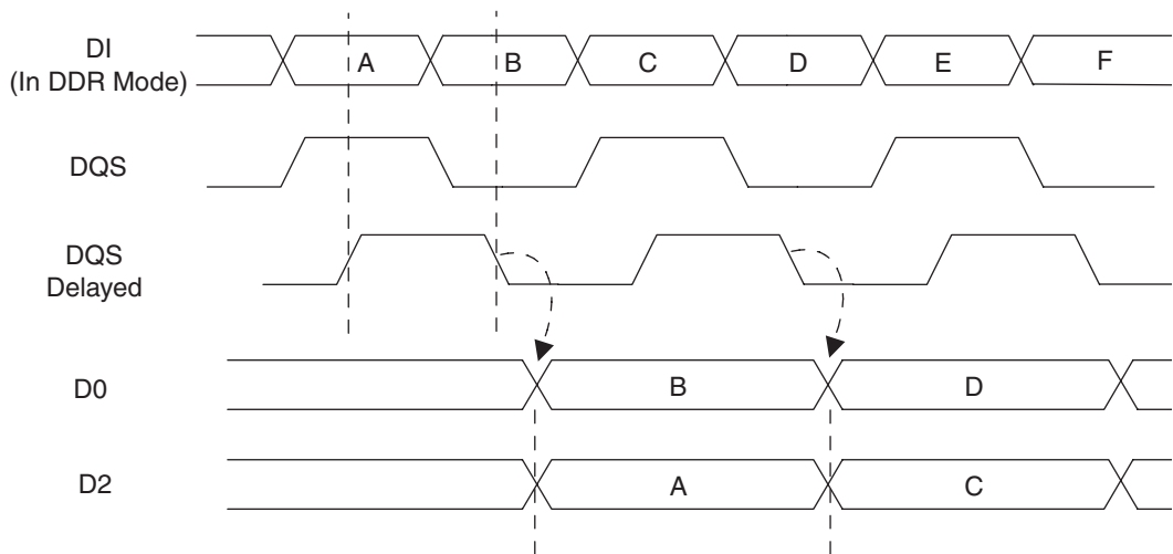
Figure 2-21. INDDRXB Primitive
