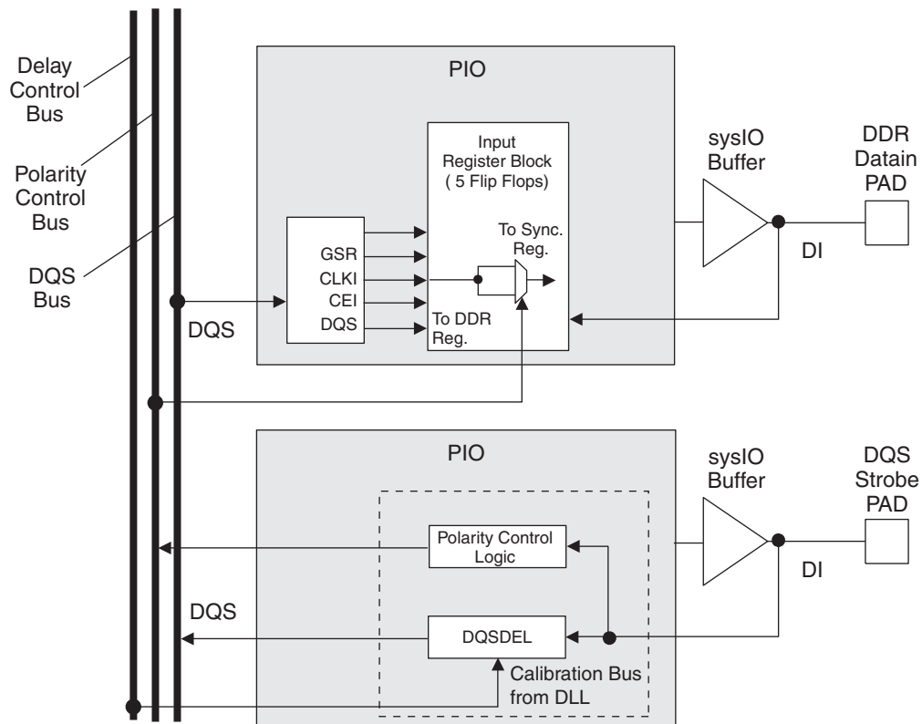
Figure 2-26. DLL Calibration Bus and DQS/DQS Transition Distribution
