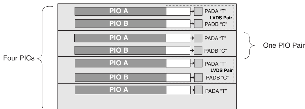
Figure 2-18. DQS Routing
