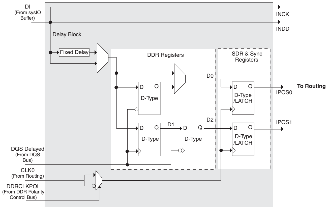
Figure 2-19. Input Register Diagram
