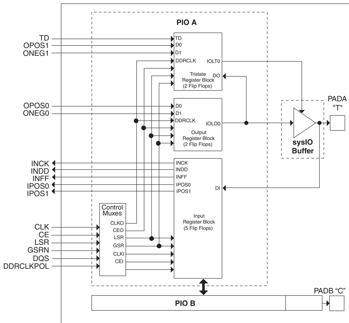
Figure 2-16. PIC Diagram
