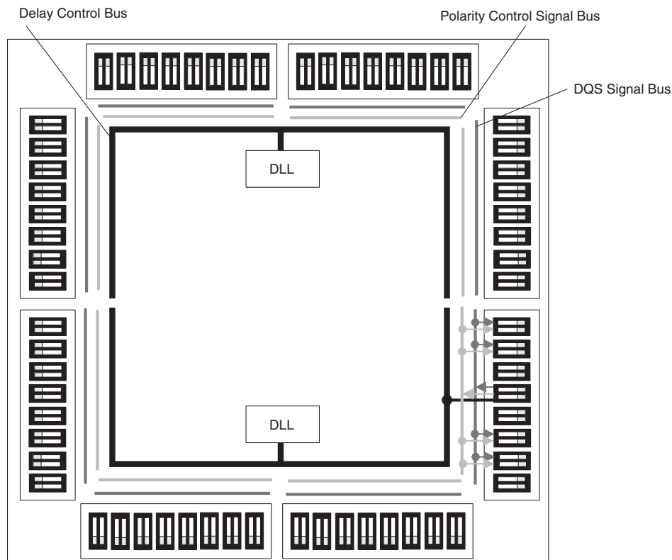
Figure 2-26. DLL Calibration Bus and DQS/DQS Transition Distribution
