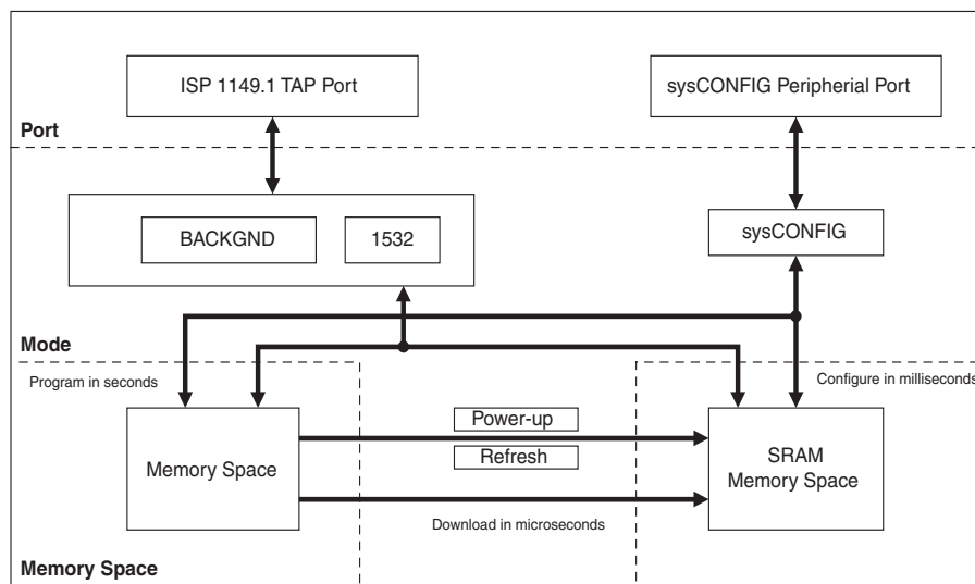
Figure 2-28. ispXP Block Diagram
