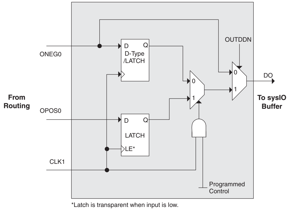
Figure 2-23. ODDRXB Primitive
