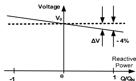
Figure 13. Droop control of the Vf inverter terminal voltage.
