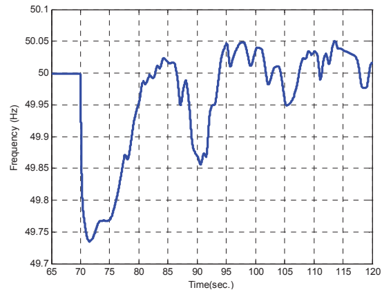
Figure 19. MG frequency.
