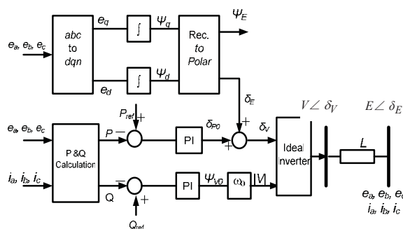
Figure 4. Simplified inverter PQ control scheme.
