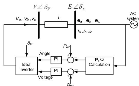
Figure 3. Basic structure of the inverter PQ control scheme.
