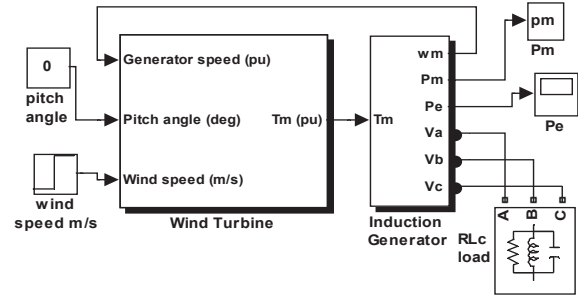
Figure 9. Wind generation system model.
