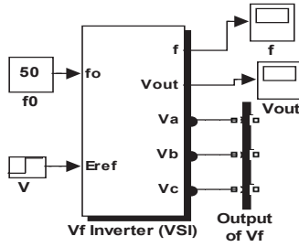
Figure 7. V_f controlled inverter.
