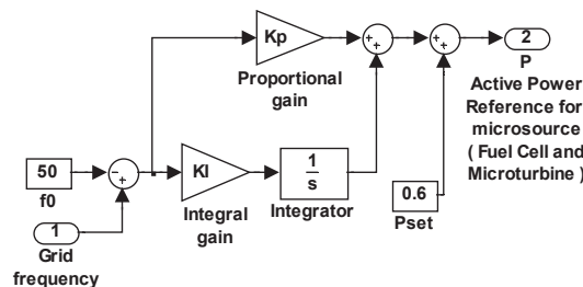
Figure 12. Control of active power of SOFC and micro turbine.
