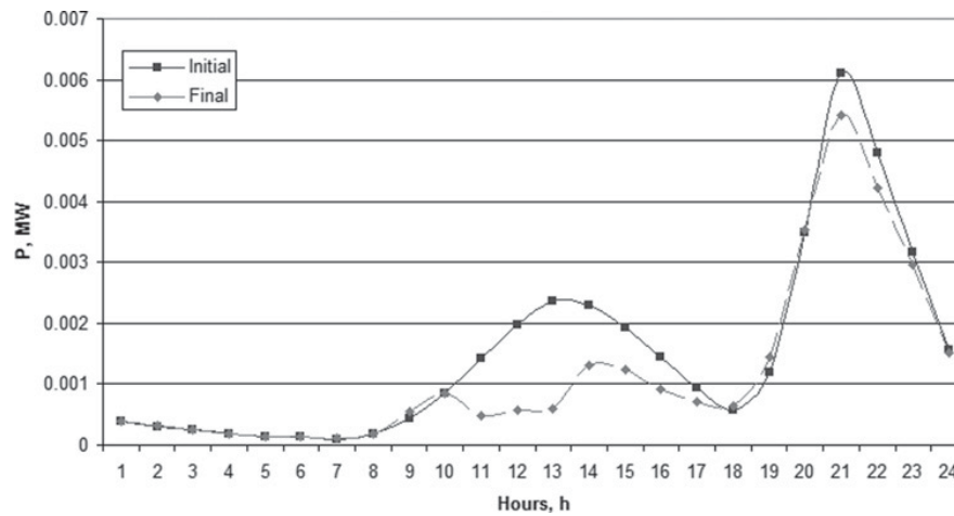
Figure 8 Active power losses in microgrid at node 64
