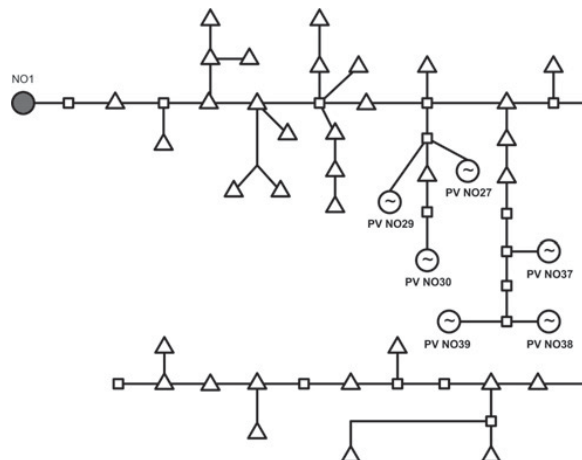
Figure 4 LV test network
