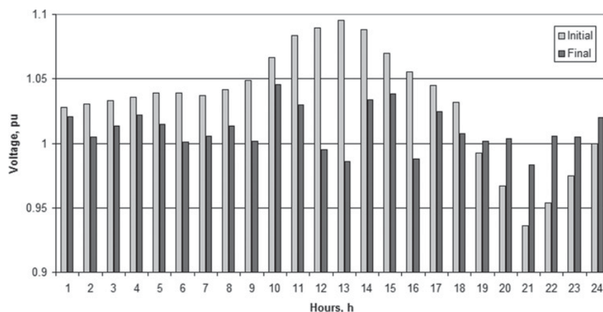
Figure 6 Maximum voltage values in microgrid at node 64
