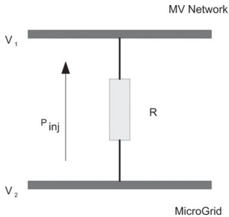
Figure 2 Example system
