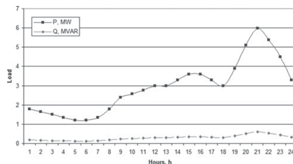
Figure 5 MV test network total load
