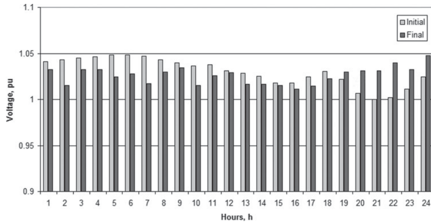
Figure 10 Maximum voltage values in the MV network
