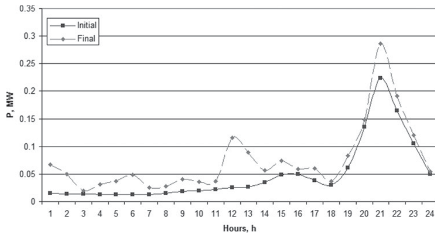
Figure 11 Active power losses in the MV network
