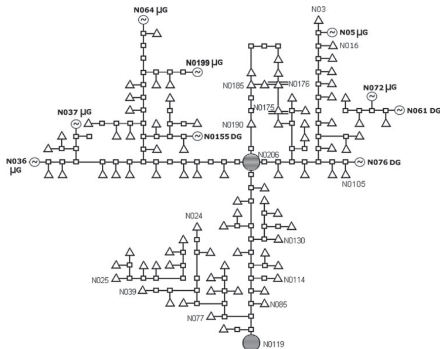
Figure 3 MV test network
