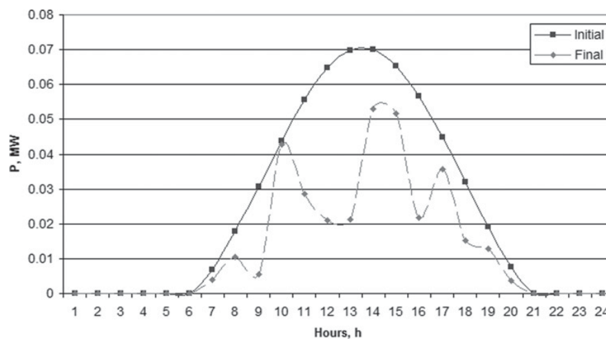
Figure 9 Total microgeneration in microgrid at node 64
