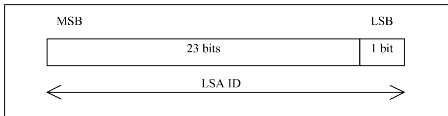
Figure 19: Structure of LSA ID
