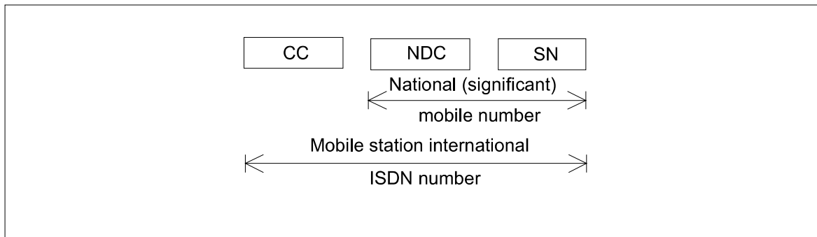
Figure 2: Number Structure of MSISDN
