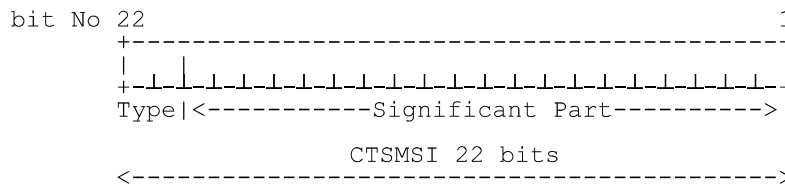
Figure 13: Structure of CTSMSI
