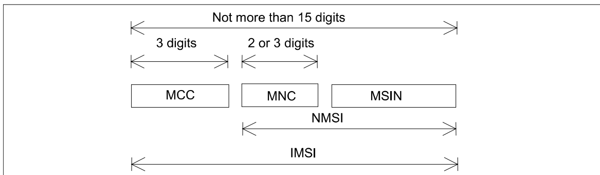
Figure 1: Structure of IMSI
