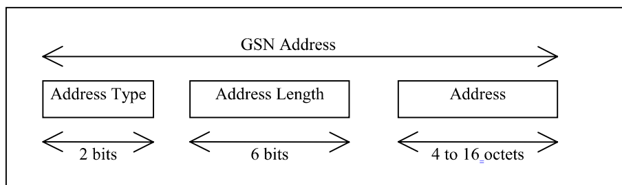
Figure 9: Structure of GSN Address
