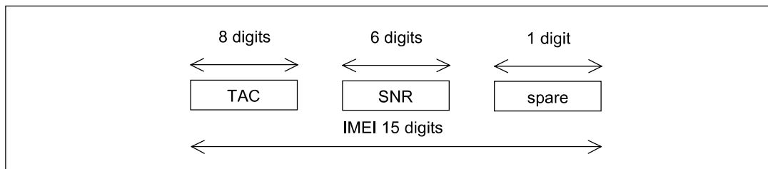
Figure 10: Structure of IMEI
