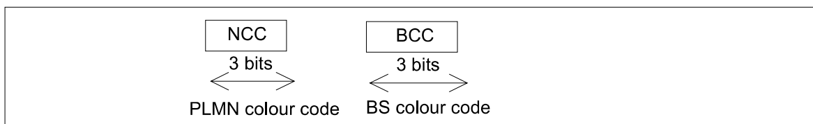
Figure 6: Structure of BSIC
