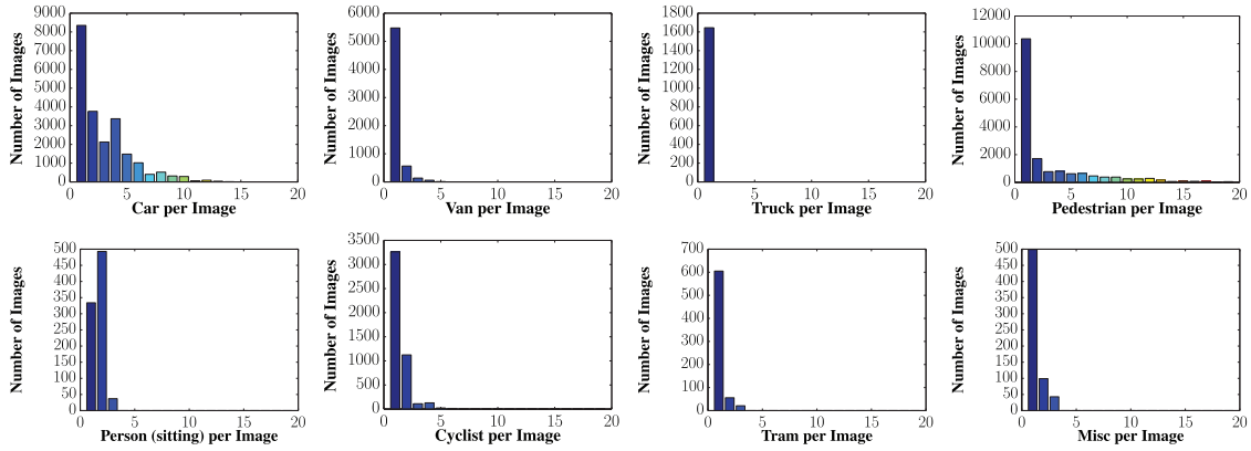
Fig. 8. Number of object labels per class and image. This figure shows how often an object occurs in an image. Since our labeling efforts focused on cars and pedestrians, these are the most predominant classes here.
