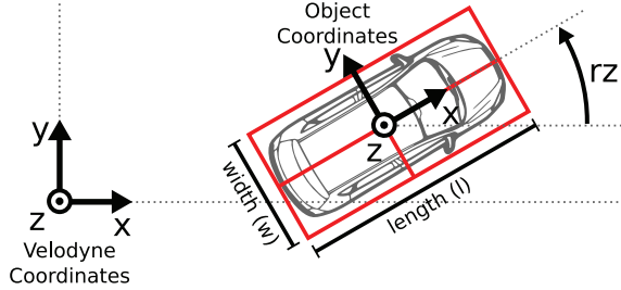
Fig. 6. Object coordinates. This figure illustrates the coordinate system of the annotated 3D bounding boxes with respect to the coordinate system of the 3D Velodyne laser scanner. In z-direction, the object coordinate system is located at the bottom of the object (contact point with the supporting surface).
