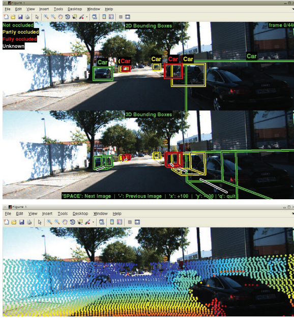
Fig. 11. Development kit. Working with tracklets (top), Velodyne point clouds (bottom) and their projections onto the image plane is demonstrated in the MATLAB development kit which is available from the KITTI website.
