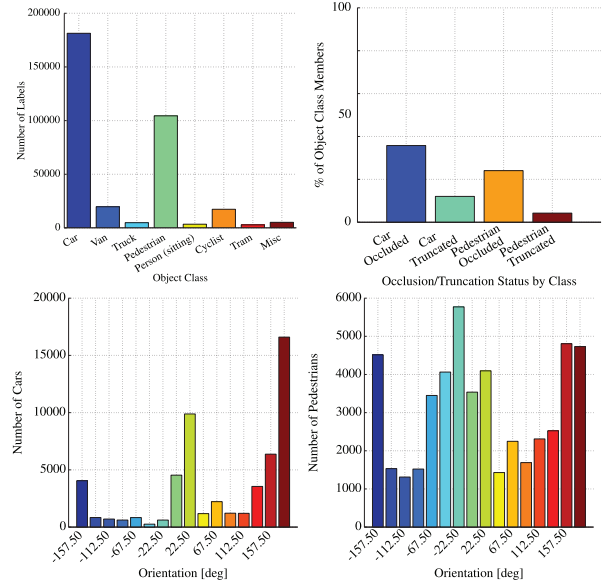
Fig. 7. Object occurrence and orientation statistics of our dataset. This figure shows the different types of objects occurring in our sequences (top) and the orientation histograms (bottom) for the two most predominant categories ‘Car’ and ‘Pedestrian’.
