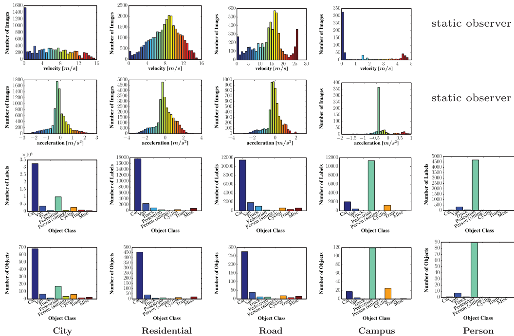
Fig. 10. Velocities, accelerations and number of objects per object class. For each scene category we show the acceleration and velocity of the mobile platform as well as the number of labels and objects per class. Note that sequences with a purely static observer have been excluded from the velocity and acceleration histograms as they don't represent natural driving behavior. The category 'Person' has been recorded from a static observer.
