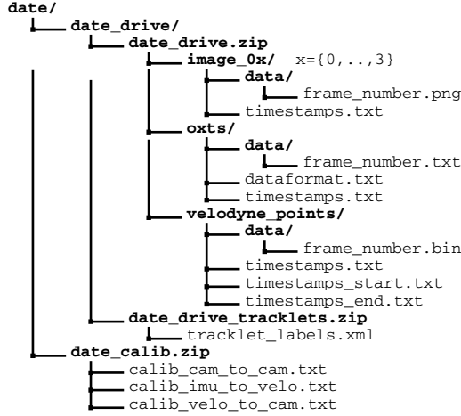
Fig. 5. Structure of the provided zip files and their location within a global file structure that stores all KITTI sequences. Here, ‘date’ and ‘drive’ are placeholders, and ‘image_0x’ refers to the 4 video camera streams.
