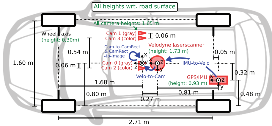
Fig. 3. Sensor setup. This figure illustrates the dimensions and mounting positions of the sensors (red) with respect to the vehicle body. Heights above ground are marked in green and measured with respect to the road surface. Transformations between sensors are shown in blue.
