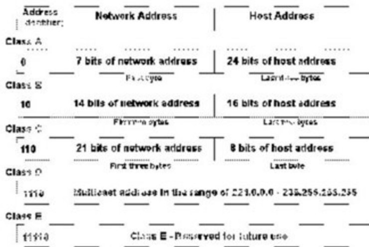
Figure 3-Address classes define the split between network and host IDs.
