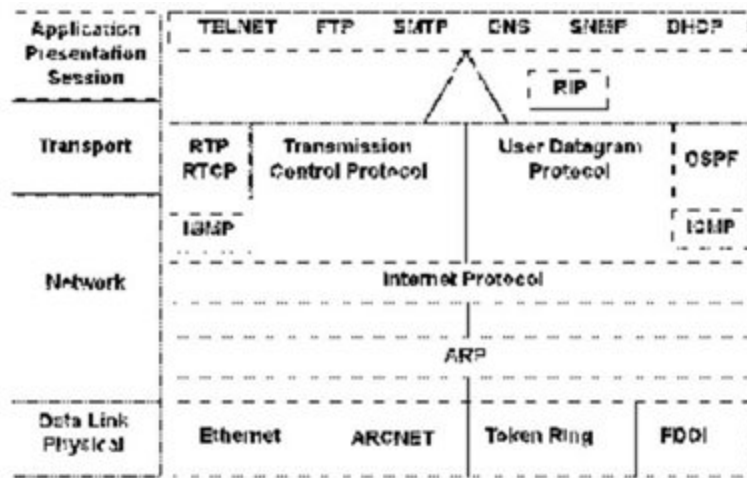
Figure 1-The TCP/IP stack is actually a set of protocols.
