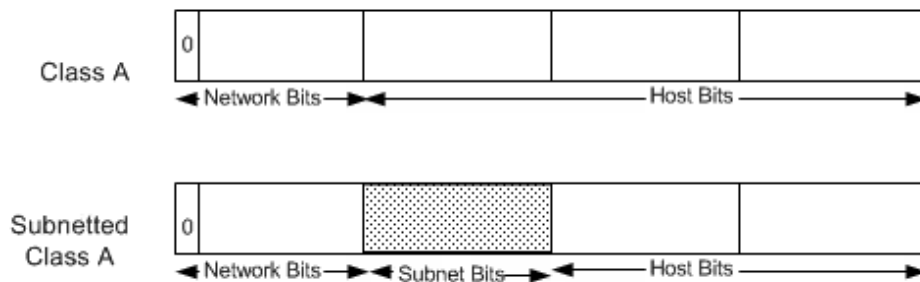
Figure 4 â "Borrowing" Bits
