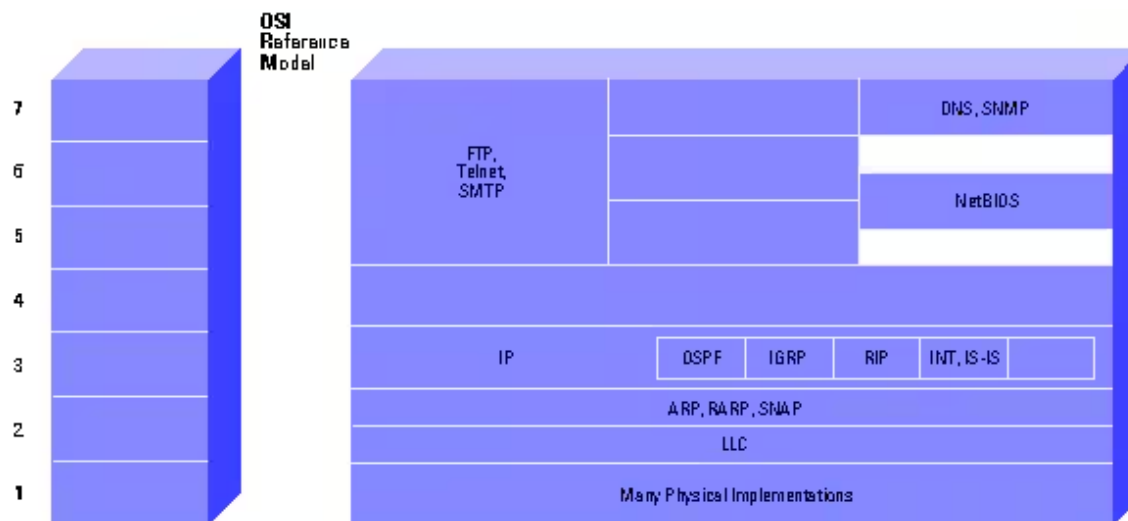
Figure 2 â Important Internet Protocols in Relation to the OSI Reference Model
