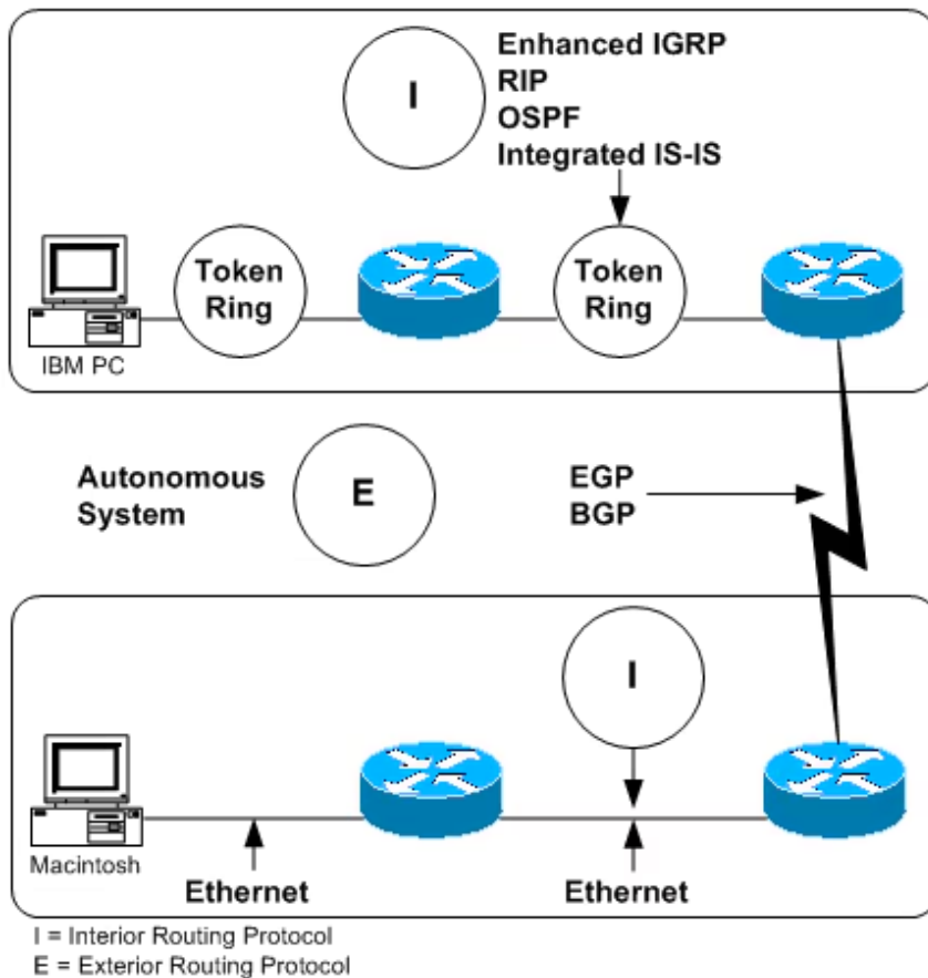
Figure 6 â Representation of the Internet Architecture
