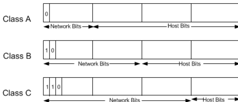
Figure 3 â Address Formats for Class A, B, and C IP Networks
