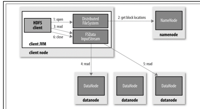
Figure 3-2. A client reading data from HDFS
