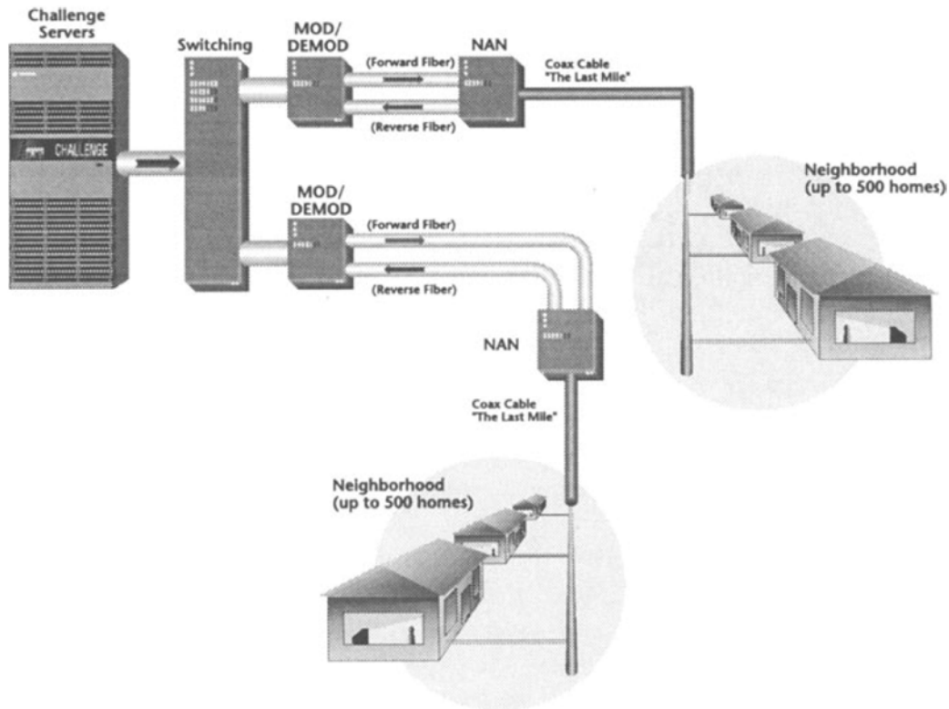
Fig. 5. Distribution network
