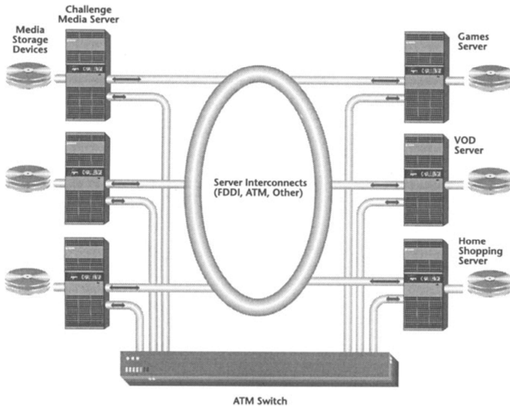
Fig. 4. Head-end server complex
