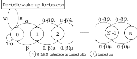
Fig. 4. State transition diagram for WLAN interface and AP buffer when PCP is not applied
