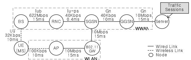
Fig. 8. Network topology
