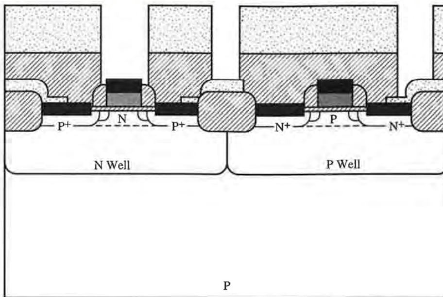
Figure 2-40 Photoresist is spun onto the wafer. Mask 12 is used to define the contact holes. The deposited \text{SiO}_2 layer is then etched to allow connections to the silicon, polysilicon and local interconnect regions.
