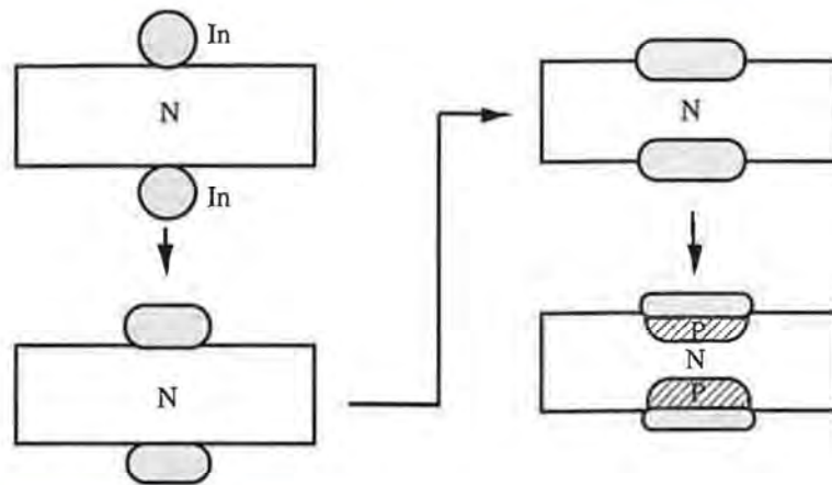
Figure 1-6 Alloy junction technology of the 1950s.
