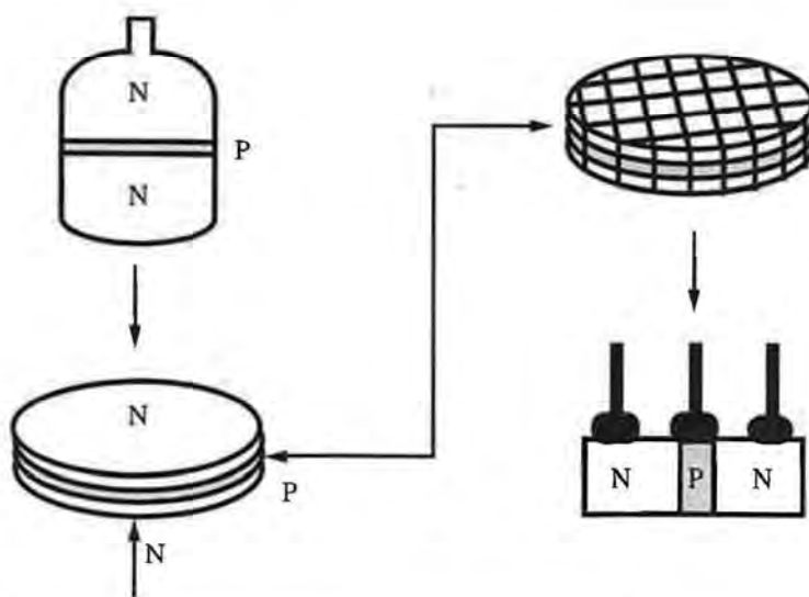
Figure 1-5 Grown junction transistor technology of the 1950s.
