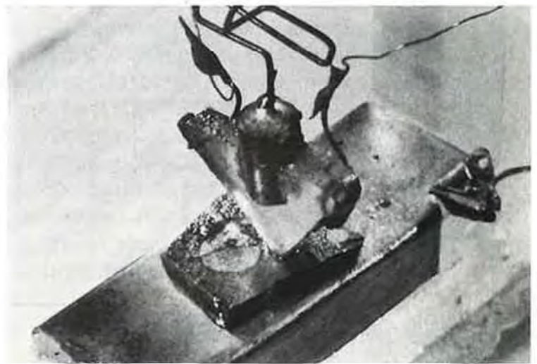
Figure 1-4 The point contact transistor invented at Bell Telephone Laboratories in 1947 by Bardeen, Brattain, and Shockley. Reprinted with permission of Lucent Technologies, Bell Labs Innovations.
