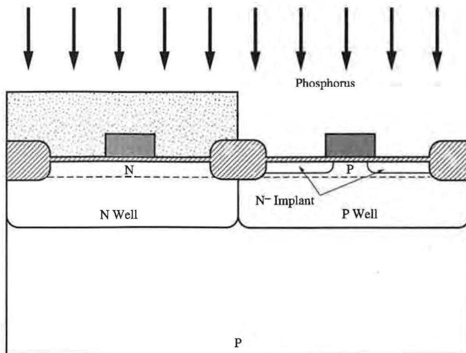
Figure 2-27 Mask 7 is used to cover the PMOS devices. A phosphorus implant is used to form the tip or extension (LDD) regions in the NMOS devices.
