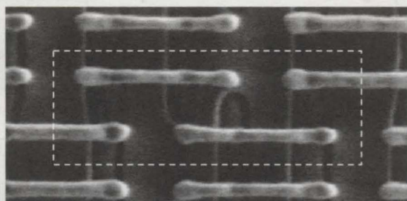
Figure 12: 0.57 \mu\text{m}^2 6-T SRAM cell at poly layer
