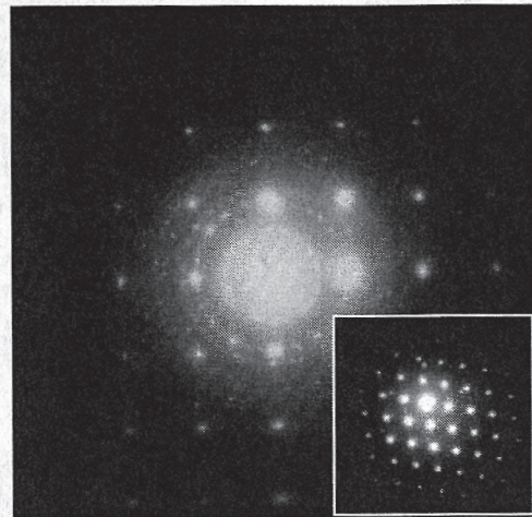
Figure 4. TEM Electron Diffraction Image of TI Transistor Channel Region (Inset – Intel Prescott, \langle 110 \rangle Channel Direction)
