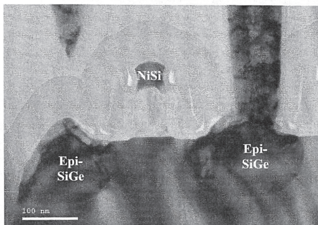
Figure 6. Intel PMOS Transistor
