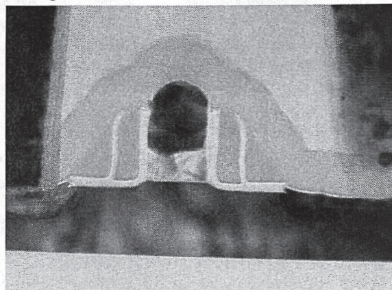
Figure 12. PMOS Transistor in AMD Athlon
