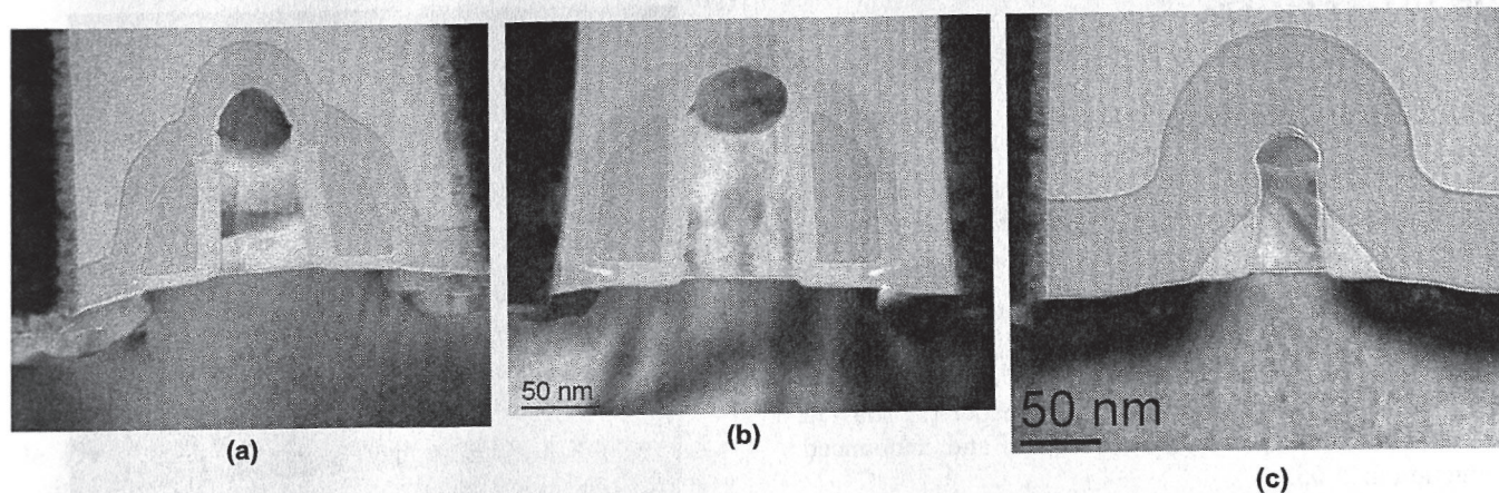
Figure 10. Transistors in (a) Xilinx Spartan-3, (b) Altera Stratix-II, (c) Transmeta Efficcon-2
