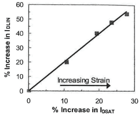
Fig. 2: Measured % improvement in PMOS linear drive ( I_{DLIN} ) vs. I_{DSAT} with increasing PMOS channel strain. I_{DLIN} gain is 2x I_{DSAT} gain due to larger sensitivity of I_{DLIN} on channel mobility.
