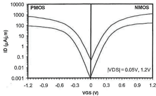
Fig. 7: NMOS and PMOS subthreshold curves.
