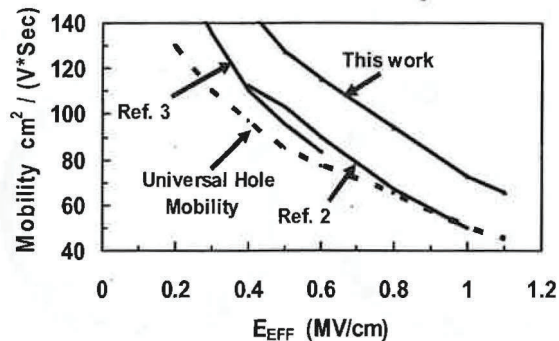
Fig. 3: Hole mobility as a function of vertical effective field for our uniaxially strained PMOS device [1] relative to conventional biaxially strained substrate techniques [2,3].
