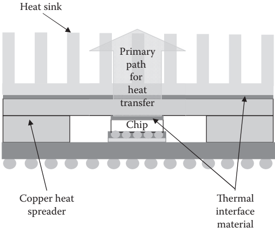
Figure 7.5 Example of a high-performance flip-chip ball grid array package with heat sink, intended for microprocessors (not to scale).
