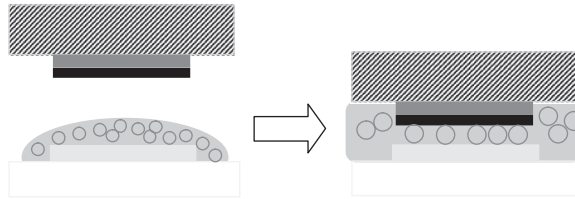
Figure 7.21 Flip-chip interconnection using anisotropic conductive adhesive.
