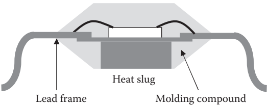
Figure 7.4 Example of a leaded plastic package with heat slug attached to die paddle (not to scale).
