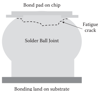
Figure 5.5 A ductile solder fatigue-induced crack due to temperature cycling (not to scale).
