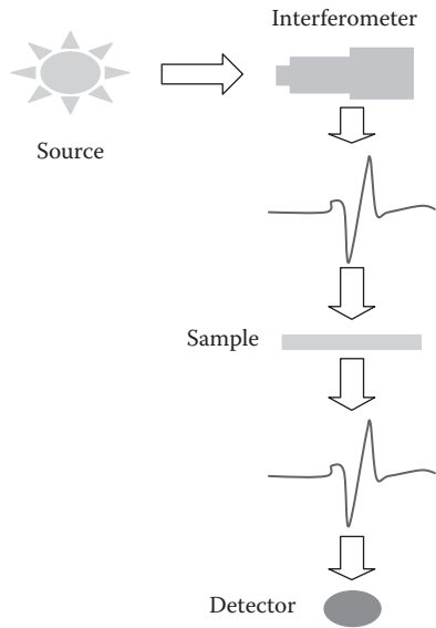
Figure B.5 Sample analysis with Fourier transform infrared spectroscopy.
