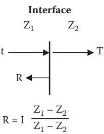
Figure A.5 Effect of acoustic impedance on coupled materials.
