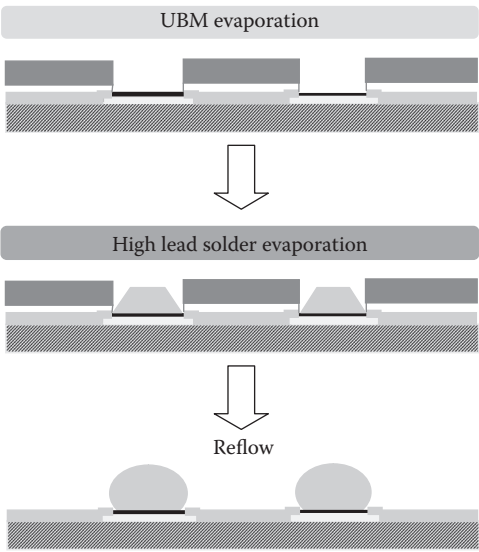
Figure 7.18 “C4” (Controlled Collapse Chip Connection) process steps.
