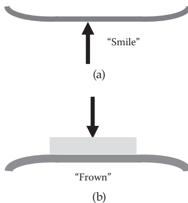
Figure 6.10 (a) Concave curvature ("smile") of substrate and package (not to scale). (b) Convex curvature ("Frown") of substrate and package (not to scale).
