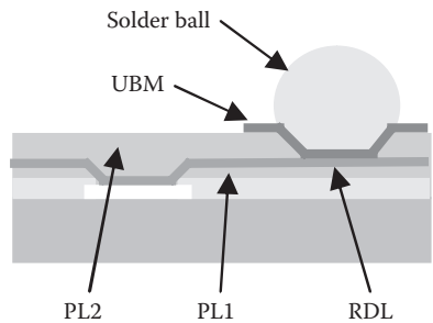
Figure 2.11 Cross section of a wafer-level chip scale package (not to scale).
