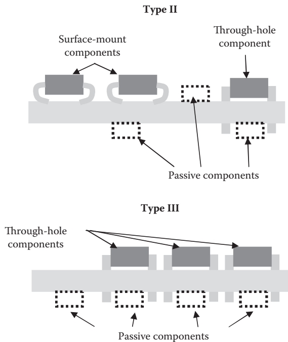
Figure 3.2 A printed circuit board populated with through-hole and surface-mount components (Type II and Type III).
