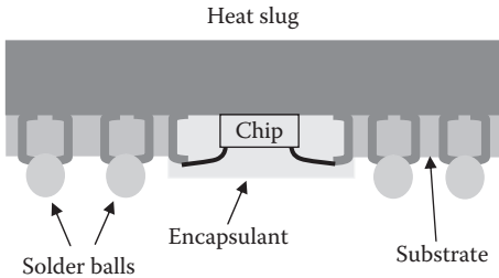
Figure 2.4 Cavity-down, thermally enhanced ball grid array (not to scale).
