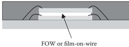
Figure 6.20 Stacked-die package using film-on-wire (not to scale).
