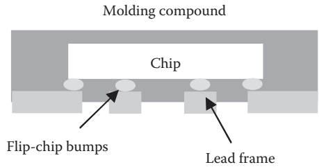
Figure 2.7 Flip-chip quad flat no lead (not to scale).
