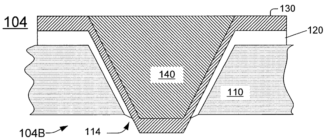
FIG. 2 PRIOR ART
