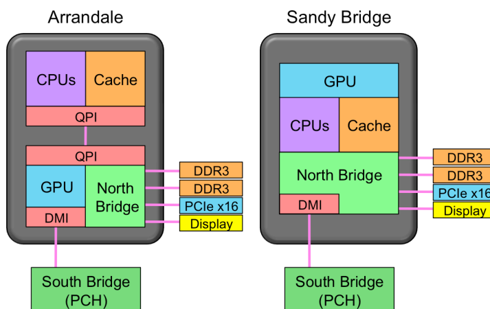
Figure 1. Arrandale versus Sandy Bridge. Arrandale combines a Westmere-based processor chip and a separate north-bridge chip in a single package. Sandy Bridge combines the processor and the north bridge, including graphics, on a single chip.
