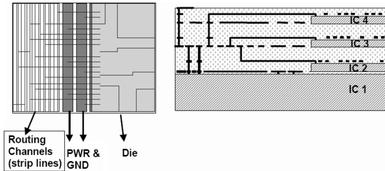
Figure 1.9 UTCS 3D routing in thin film dielectric [8].
