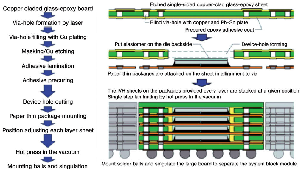
Figure 1.14 Toshiba system block module process flow [15].
