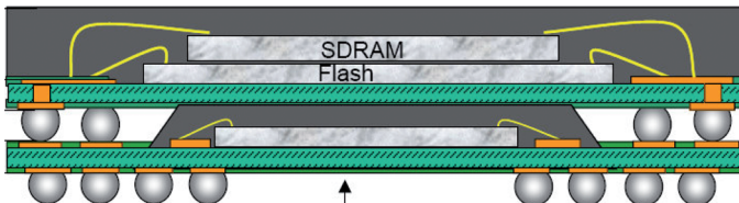
Figure 1.6 Typical Amkor PoP.
