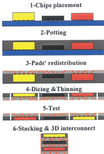
Figure 1.13 Leti – 3D plus “re-built wafer” technology [14].
