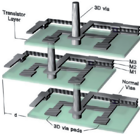
Figure 1.1 3D wafer level stacking using through silicon interconnect vias. Figure courtesy of Professor Duncan Elliott, Department of Electrical and Computer Engineering, University of Alberta.
