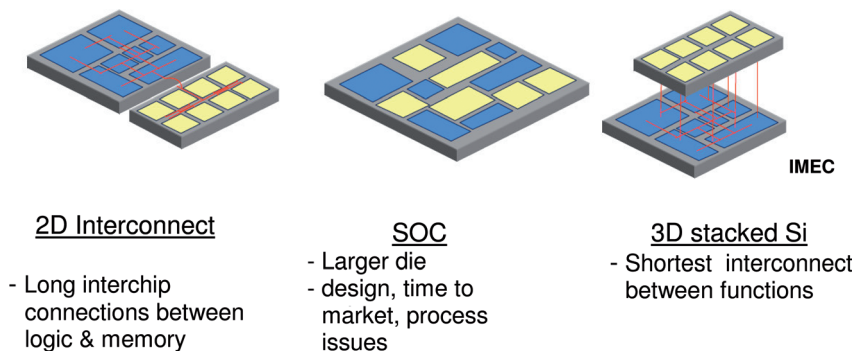
Figure 1.2 2D vs SOC vs 3D. Figure courtesy Professor Eric Beyne, MEC.
