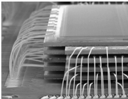
Figure 1.4 Wire bonded chips stacked in 3D package.
