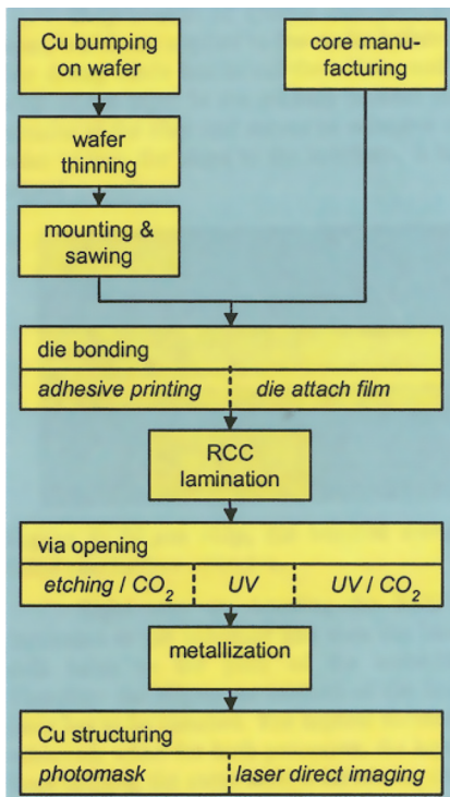
Figure 1.12 Fraunhofer/IZM chip in polymer process flow [13].
