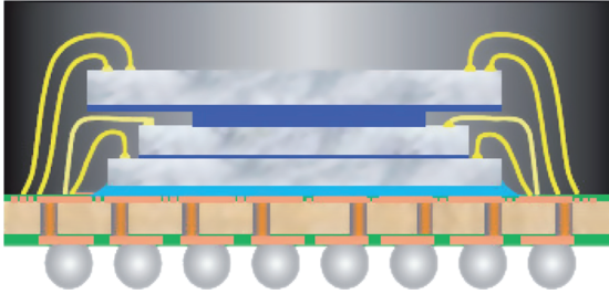
Figure 1.5 3D stacked die BGA package.
