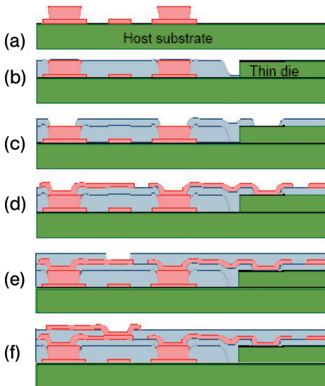
Figure 1.10 UTCS process sequence:
