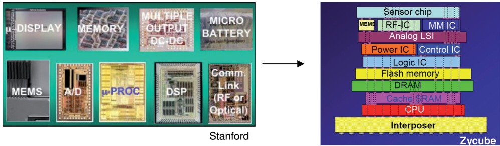
Figure 1.3 The “Holy Grail” – 3D stacking for “heterogeneous integration.” Figures courtesy of Stanford University, CA, and Zycube, Japan.
