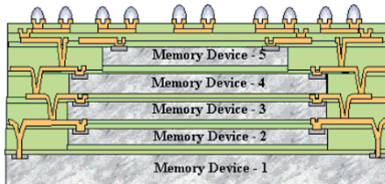
Figure 1.11 Fujitsu chip scale module memory stack [11].
