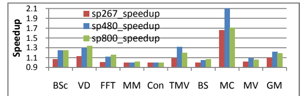
Figure 14. The speedups from CPU pre-execution for GPUs running at different frequencies and the normalized execution time without pre-execution.
