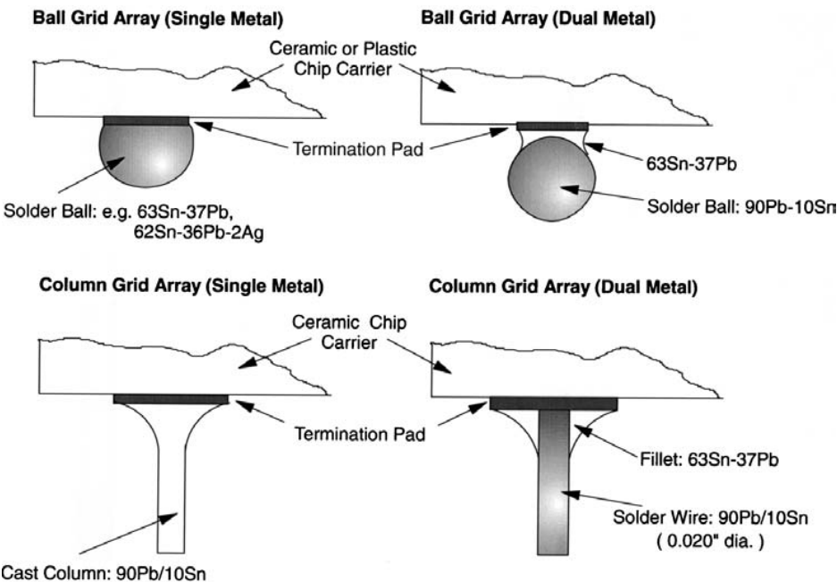
FIG. 9 Illustration depicting typical ball and column grid array terminations.
