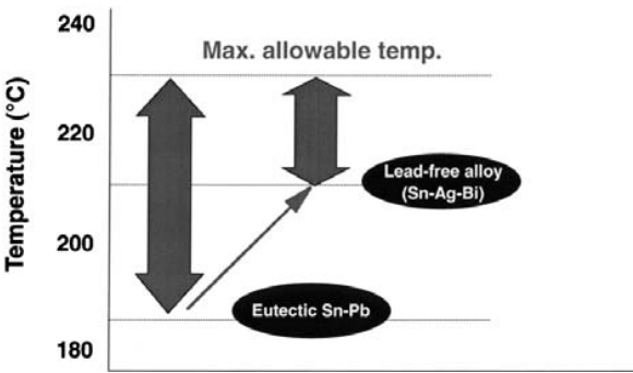
FIG. 10 Process window comparison between eutectic Sn–Pb and Sn–Ag–Bi solder alloys. (From Ref. 56.)
