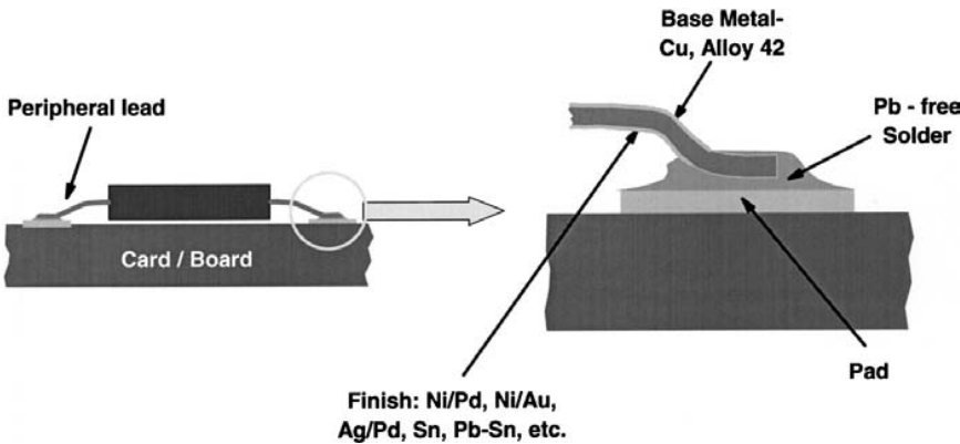
FIG. 8 Illustration depicting typical wetting characteristics of peripherally leaded components with lead-free solders.
