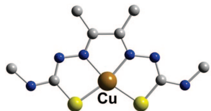
Figure 6. Cu-ATSM (L9).
