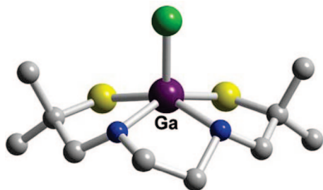
Figure 32. Ga-BAT-TM (L4).
