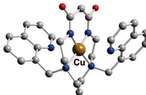
Figure 16. Cu-L35.
