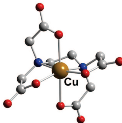
Figure 7. Cu-EDTA (L10).
