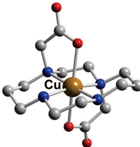
Figure 20. Cu-L51.
