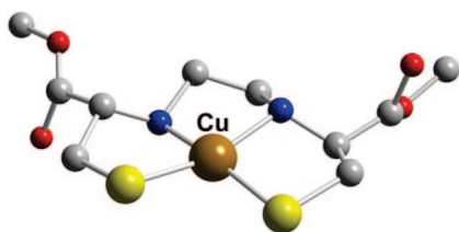
Figure 4. Cu-L6.
