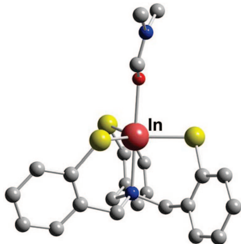
Figure 45. In-L2·DMF.
