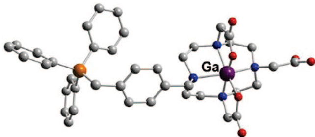
Figure 40. Ga-DO3A-TPP (L44).
