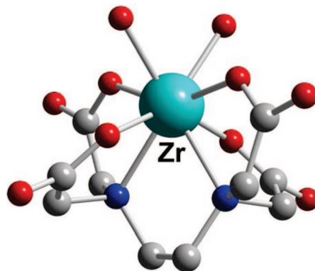
Figure 63. Zr-EDTA (L10).
