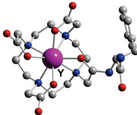
Figure 61. Y-DOTA-D-Phe-NH 2 (L40).
