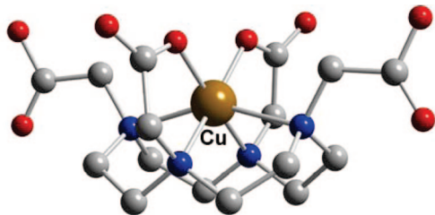
Figure 17. Cu-DOTA (L39).
