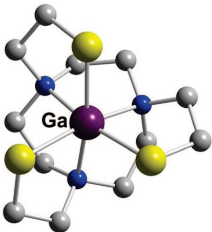
Figure 37. Ga-TACN-TM (L27).
