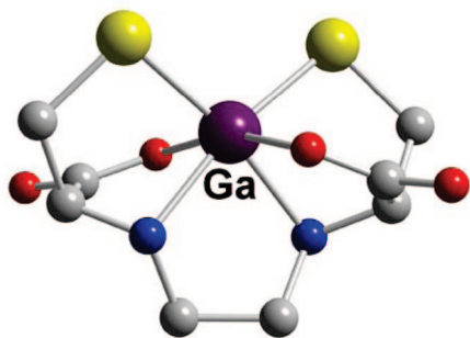
Figure 33. Ga-EC (L5).
