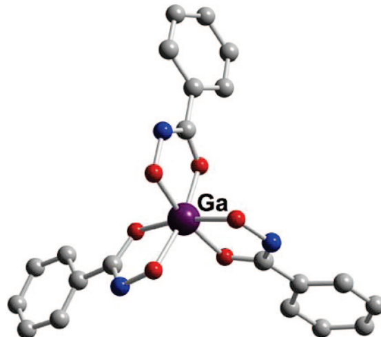
Figure 43. Ga-tris(benzohydroxamate).
