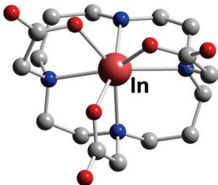
Figure 55. In-TE3A (L53).
