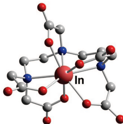
Figure 48. In-DTPA (L12).
