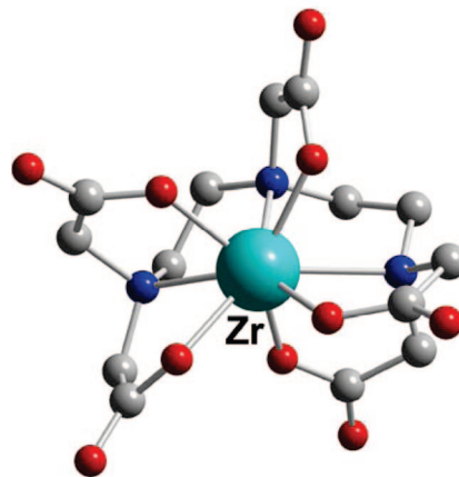
Figure 64. Zr-DTPA (L12).
