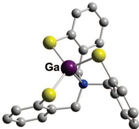
Figure 31. Ga-L2.
