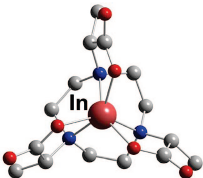
Figure 51. In-TACN (L26)-tris(2'-methylcarboxymethyl).
