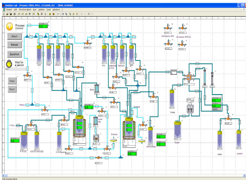
Fig. 2. Schematic of the Eckert & Ziegler module setup that identifies all valves and vials.
