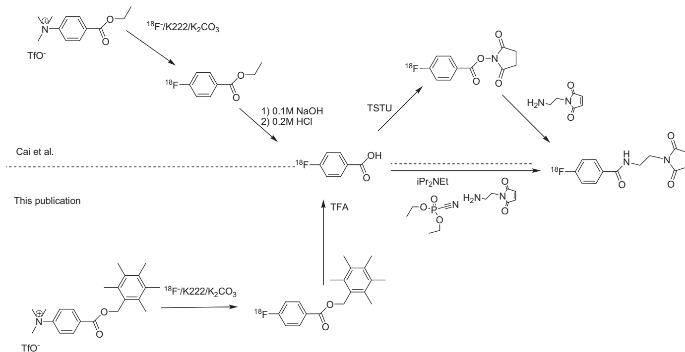
Fig. 1. Scheme of the chemical transformations during the radiochemical synthesis. The steps above the dashed line indicate the procedure of Cai et al. (2006), while those below the line are the steps of the procedure described in this manuscript.
