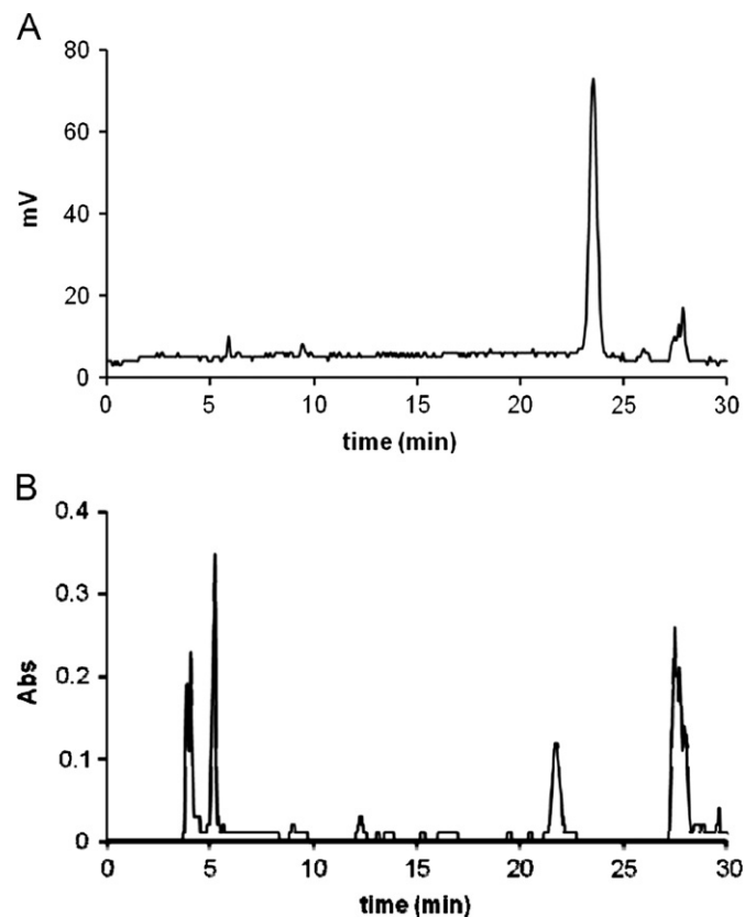
Fig. 3. Example HPLC chromatogram of [ ^{18} F]FBEM purification; panel A: radiochemical trace and panel B: UV trace at 254 nm.
