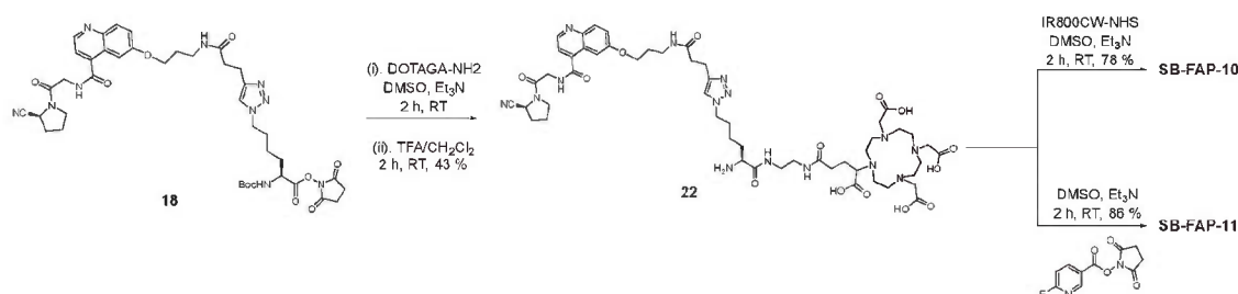
Scheme 12. Synthesis of SB-FAP-10 and SB-FAP-11.
