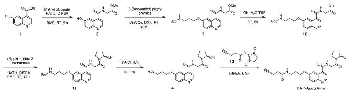
10 Scheme 4. Synthesis of FAP-Acetylene 1.
