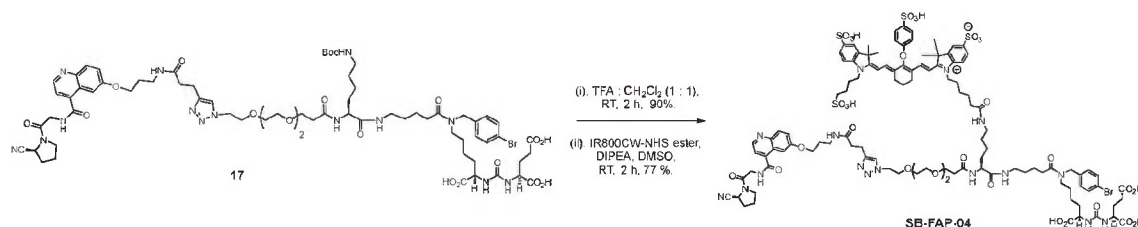
20 Scheme 8. Synthesis of SB-FAP-04.
