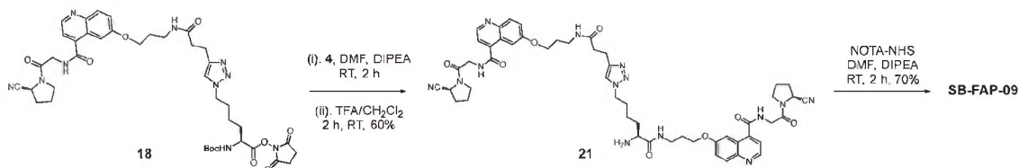
Scheme 11. Synthesis of SB-FAP-09.
