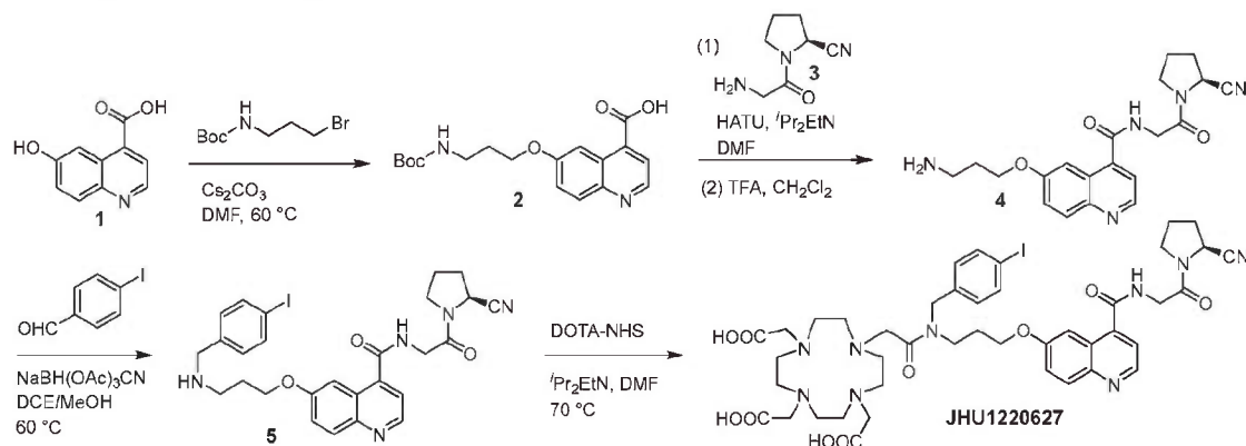
Scheme 1. Synthesis of JHU1220627.
