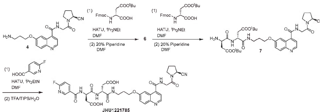
Scheme 2. Synthesis of JHU1221785.
