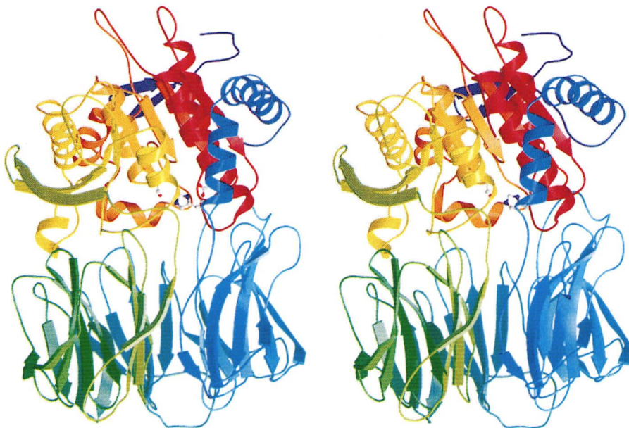
Figure 2. Stereo Representation of the Structure of Prolyl Oligopeptidase
