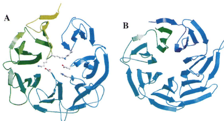
Figure 4. Comparison of the Fold of the Noncatalytic Domain of Prolyl Oligopeptidase with a Typical \beta -Propeller Structure
