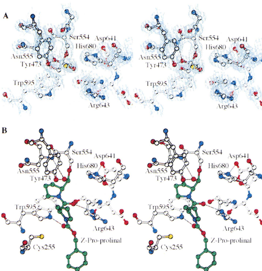
Figure 5. Stereo View of the Active Site of Prolyl Oligopeptidase
