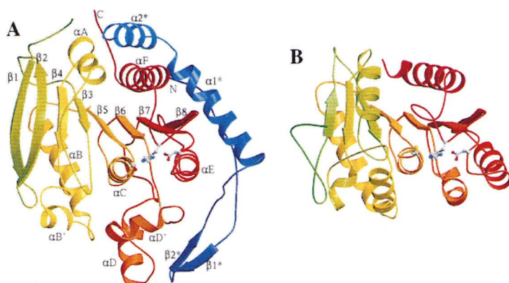
Figure 3. Comparison of the Fold of the Catalytic Domain of Prolyl Oligopeptidase with a Typical \alpha/\beta Hydrolase Domain Enzyme
