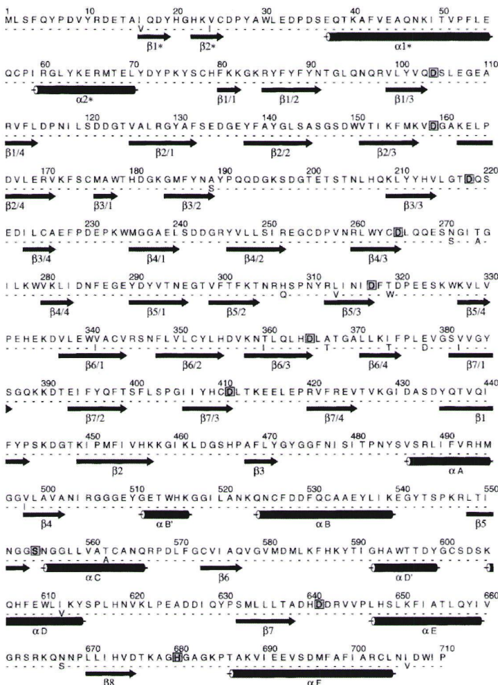
Figure 1. Amino Acid Sequence and Secondary Structure of Prolyl Oligopeptidase
