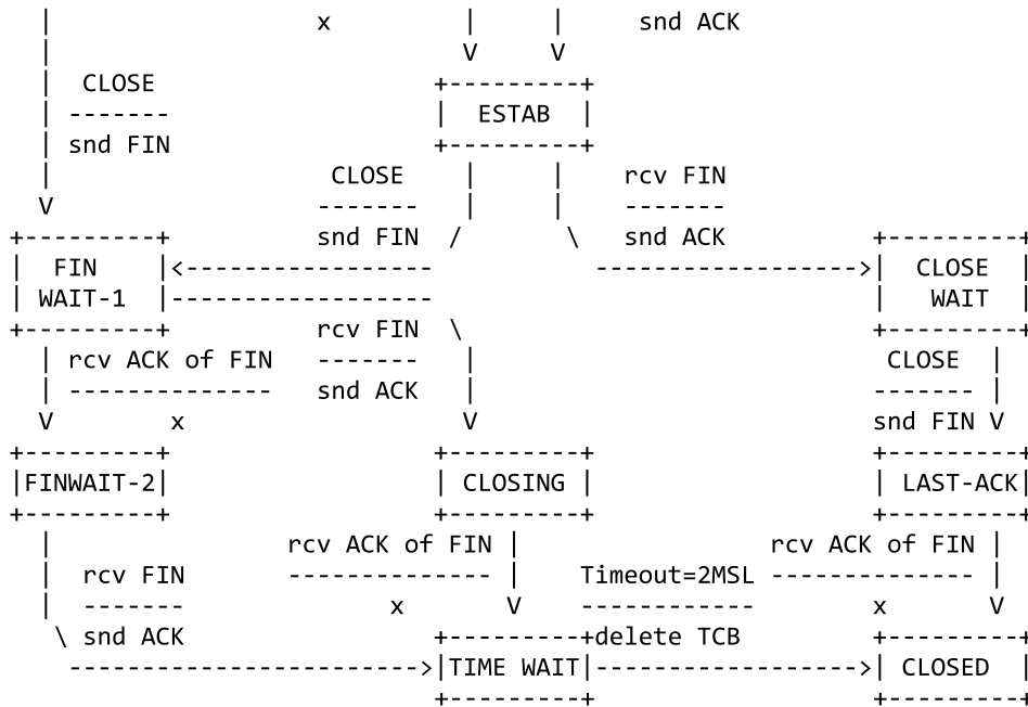
TCP Connection State Diagram Figure 6.
