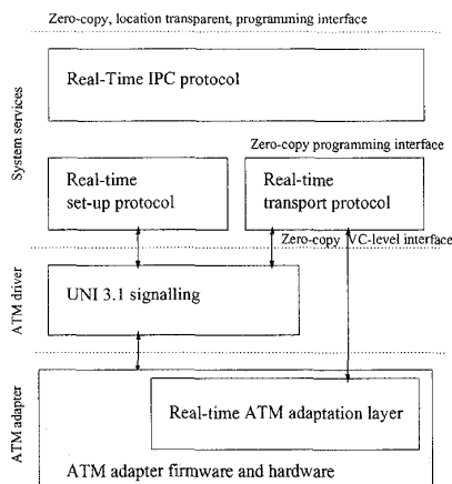
Figure 1. Architecture of the communication system.
