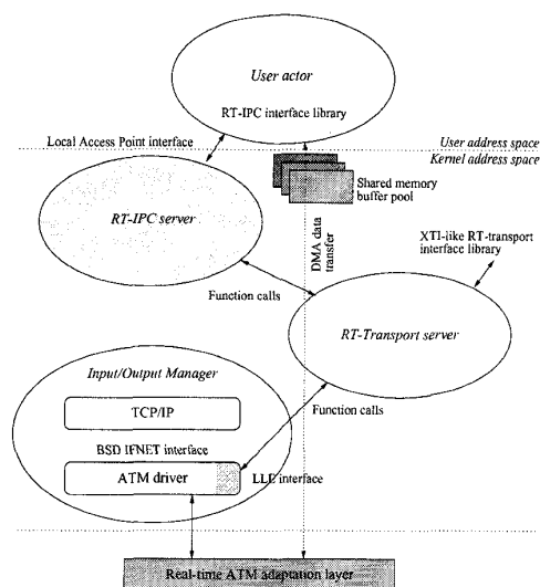
Figure 2. Implementation of the real-time IPC system.
