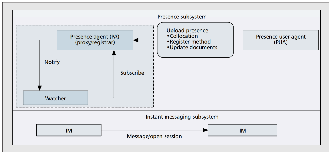
■ Figure 2. SIMPLE components.
