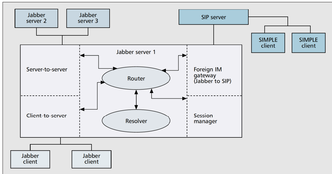
■ Figure 3. Jabber architecture.
