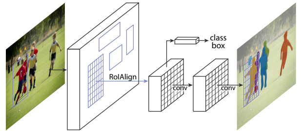
Figure 1. The Mask R-CNN framework for instance segmentation.
