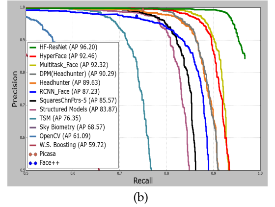
Fig. 7. Face Detection performance evaluation on (a) the AFW dataset, (b) the PASCAL faces dataset. The numbers in the legend are the mean average precision (mAP) for the corresponding datasets.
