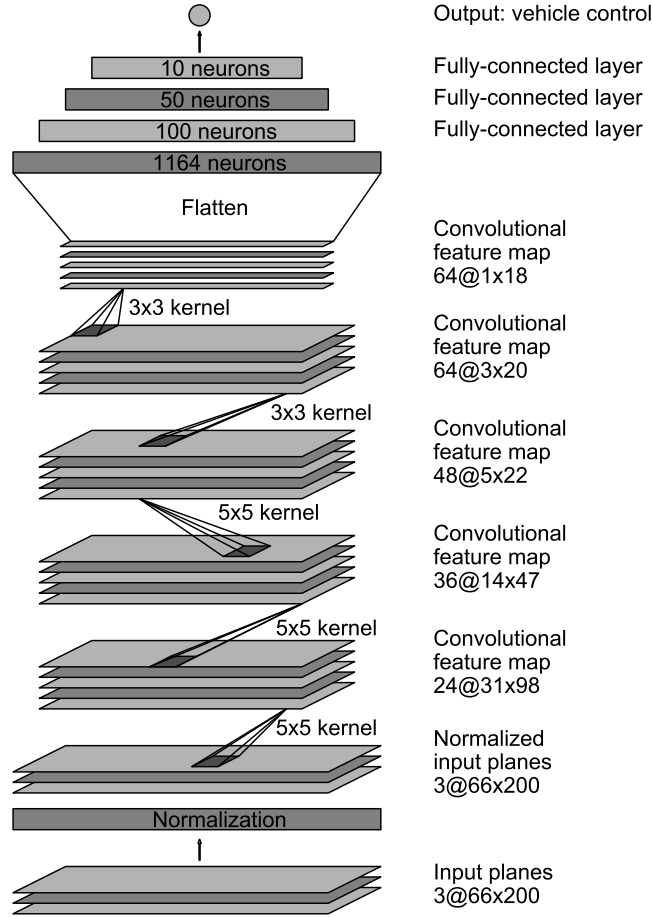
Figure 1: PilotNet architecture.
