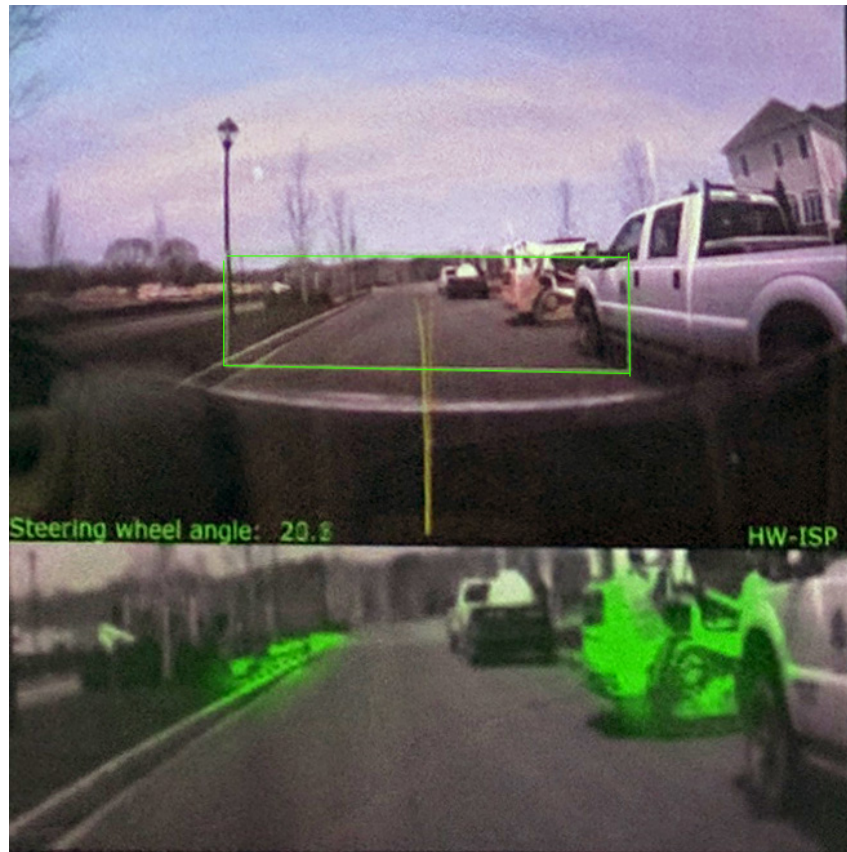
Figure 6: The PilotNet monitor from Figure 5 above
