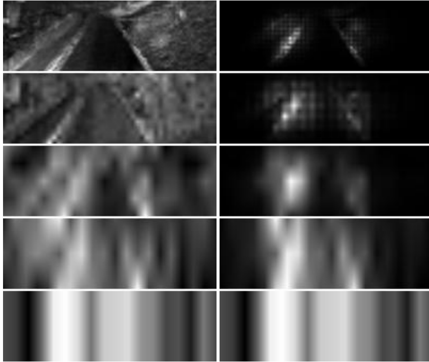
Figure 3: Left: Averaged feature maps for each level of the network. Right: Intermediate visualization mask for each level of the network.
