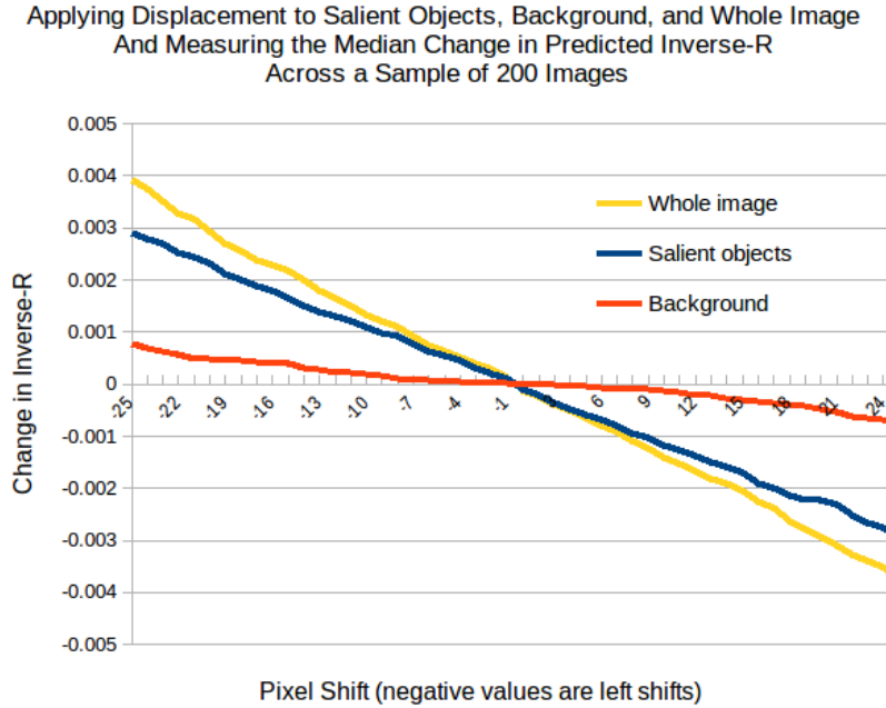
Figure 8: Plots of PilotNet steering output as a function of pixel shift in the input image.
