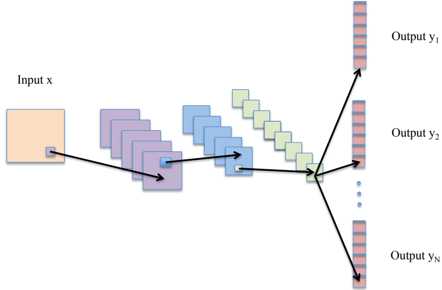
Figure 1: An example of a convolutional neural network. The network takes a single input and computes N outputs. Each output is associated with a different loss function. The biggest part of the network is shared, while task specific parts exist only close to the output of the network.
