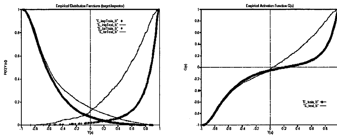
Figur 9 Empirical distribution functions after bias compensation
