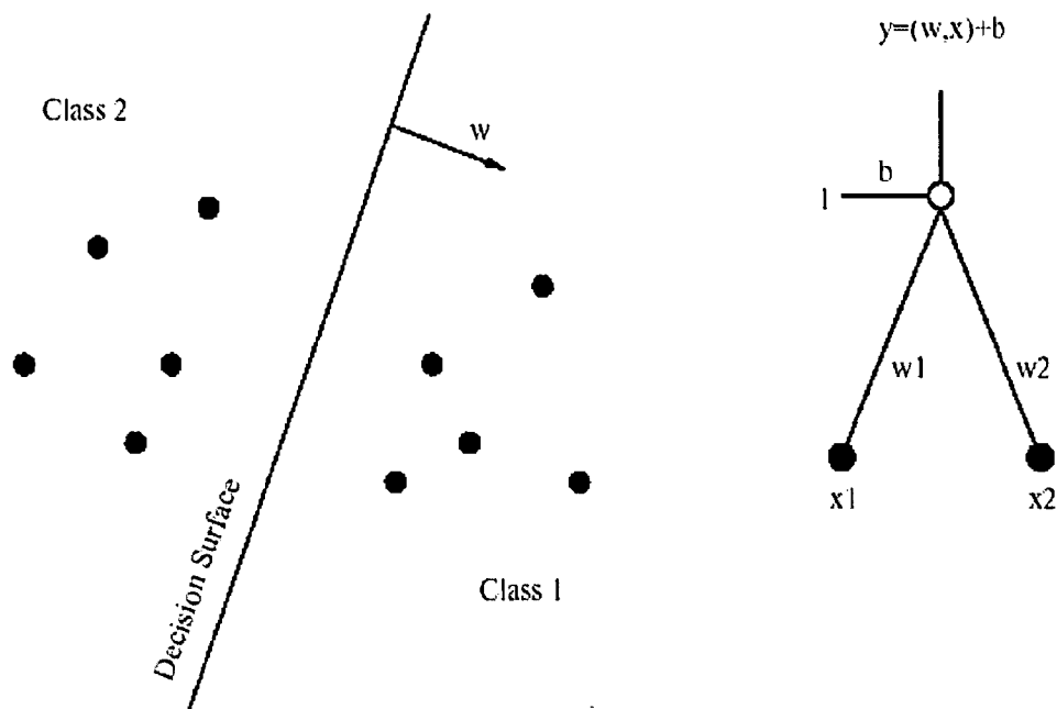
Figure 6: The perceptron (right) forms a hyper plane and classifies samples according to which side of the hyper plane they fall.
