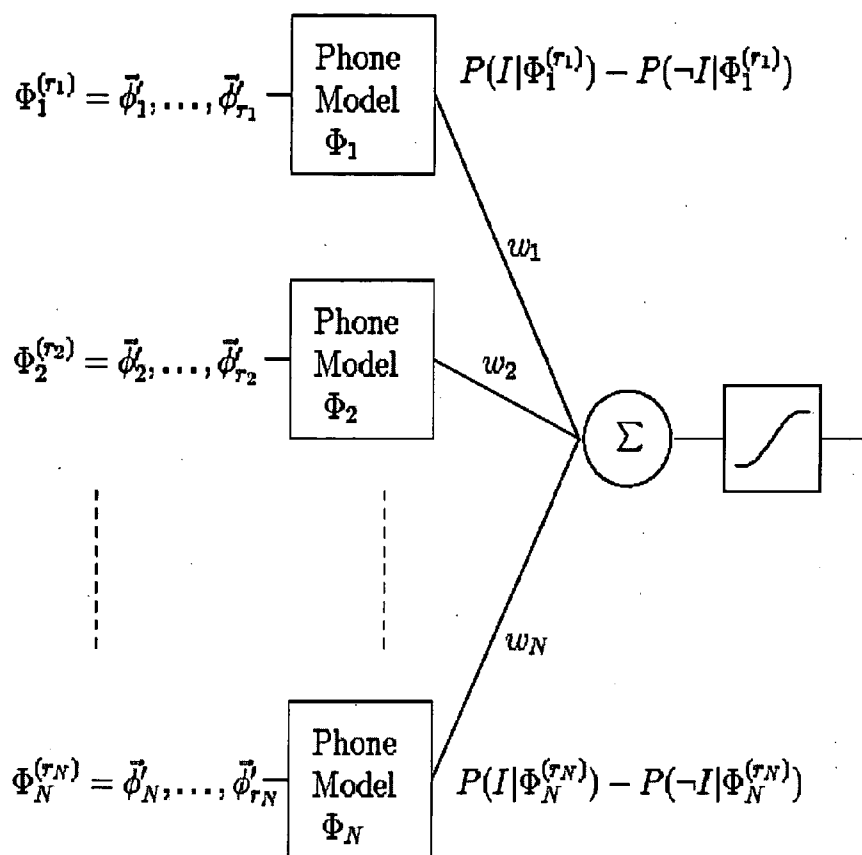
Figure: 2 A super classifier
