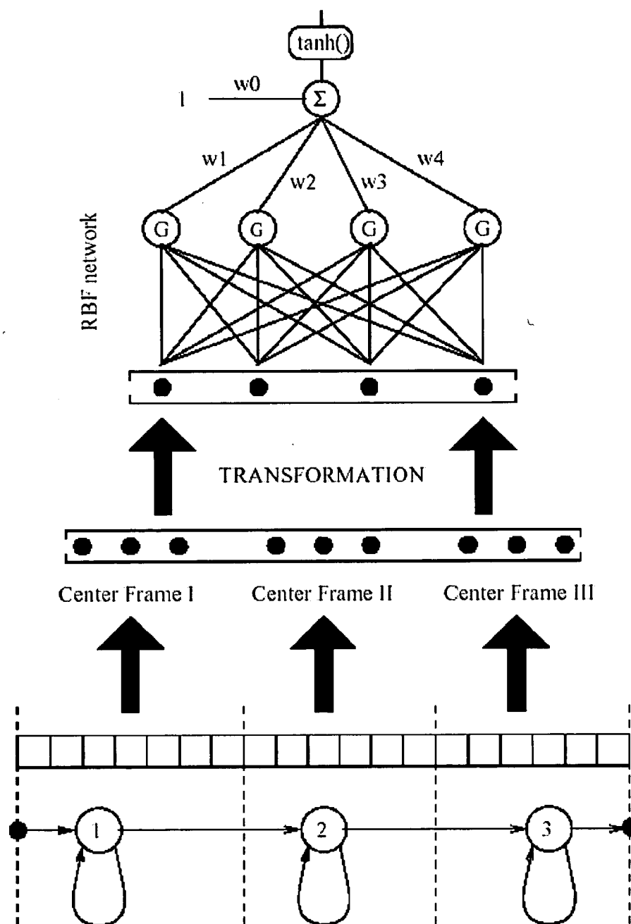
Figur 7: RBF network
