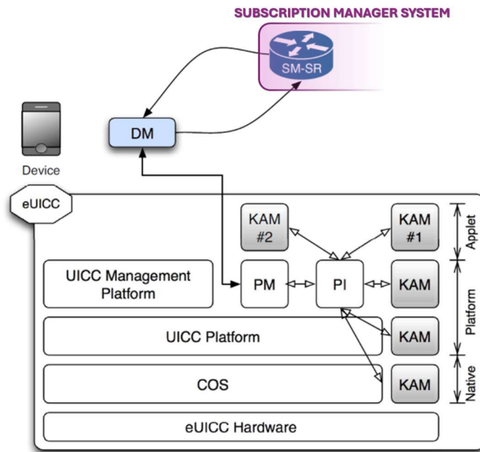
Fig. 5. Internal Architecture of eUICC
