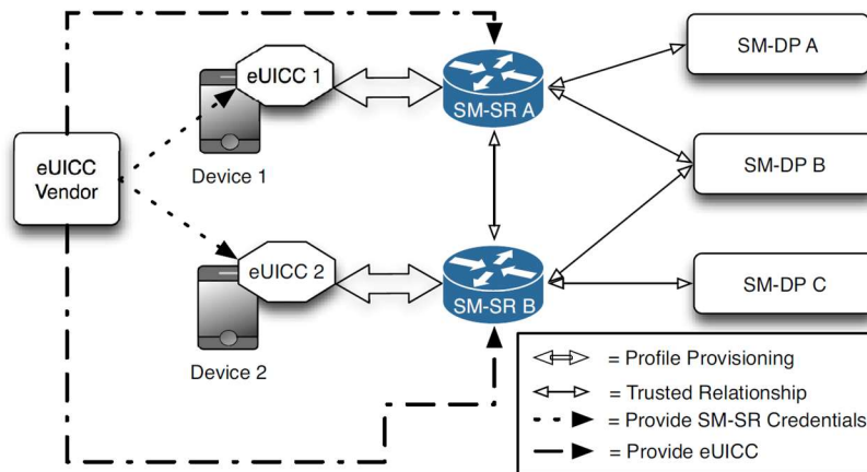
Fig. 1. eUICC Profile Ecosystem
