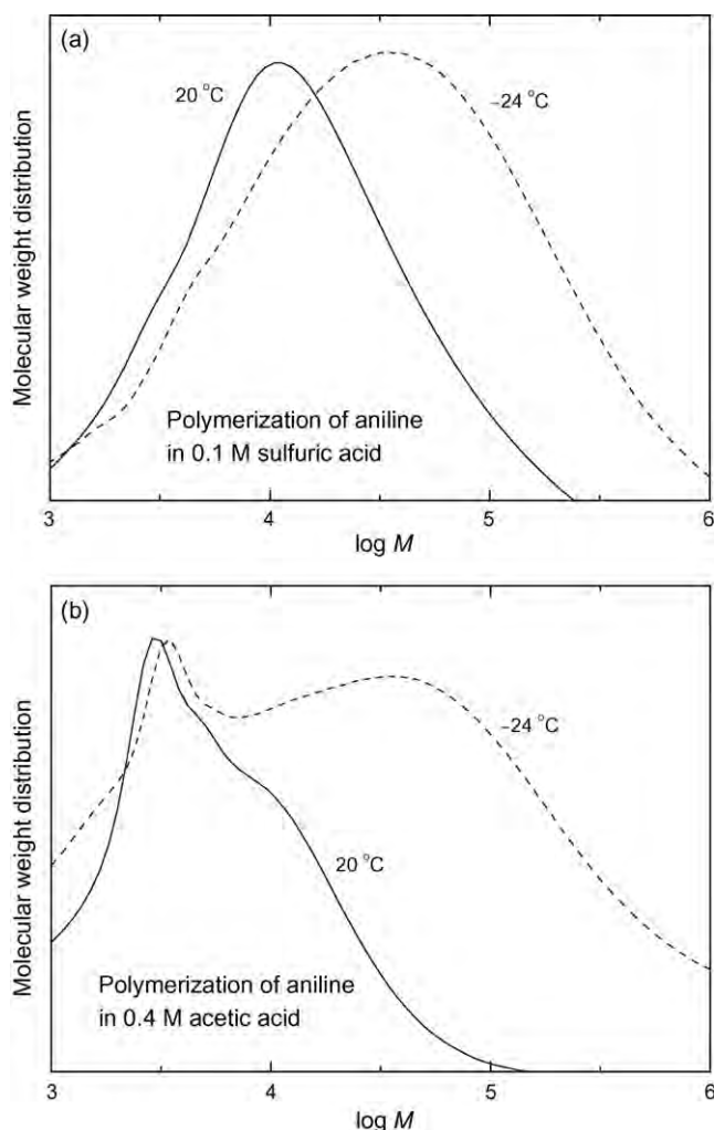
Fig. 5. Weight distributions of the molecular weight of PANI prepared in a liquid reaction mixture at 20 °C and in the frozen mixture at –24 °C (a) in 0.1 M sulfuric acid and (b) in 0.4 M acetic acid.
