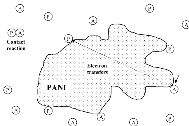
Fig. 8. A PANI chain growing in contact with PANI particles (marked by full arrow) adds an aniline monomer molecule (A) as a new constitutional unit. The electrons abstracted during the formation of the chemical bond incorporating the aniline molecule are transferred to the oxidant, peroxydisulfate molecule (P), which is reduced to sulfate. Any oxidant molecule in contact with PANI particles can accept electrons, which are transported through the conducting PANI phase (broken arrow) from the locus of polymerization. Aniline can also react with peroxydisulfate in the classical way, by exchanging electrons after physical contact between the molecules.
