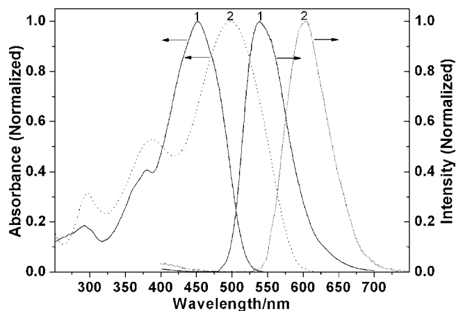
Fig. 1. Normalized absorption and fluorescence spectra of 1 and 2 in dichloromethane (10 \mu\text{M} ).
