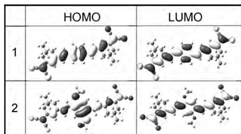
Fig. 4. HOMO and LUMO orbitals in the optimized ground-state structures of 1 and 2 .
