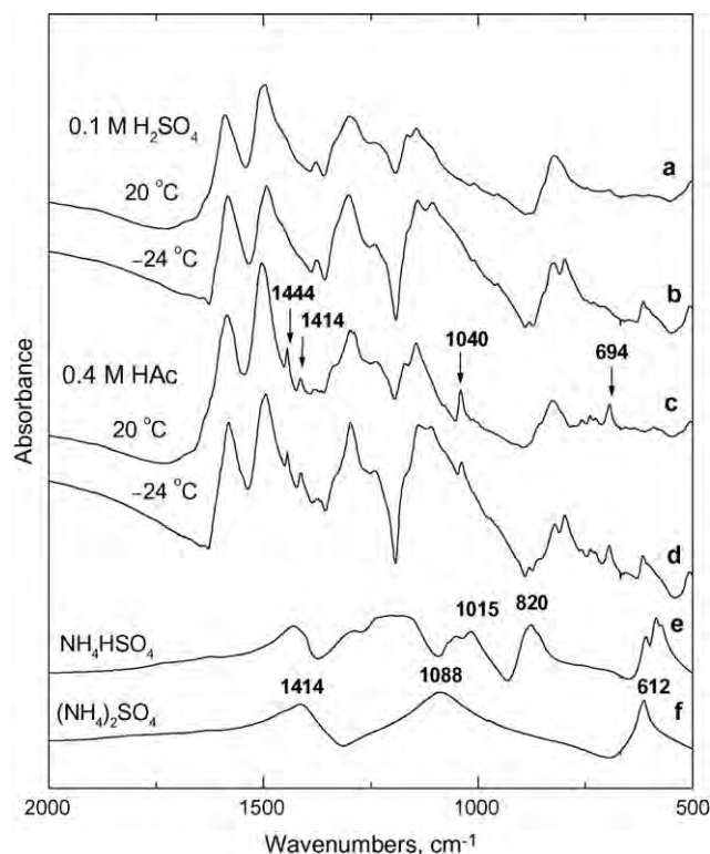
Fig. 6. The FTIR spectra of PANI bases obtained after deprotonation of the samples prepared in a liquid reaction mixture at 20 °C in 0.1 M sulfuric acid (a) and in 0.4 M acetic acid (c), the spectra of the deprotonated samples polymerized in frozen mixtures, in ice, at –24 °C in 0.1 M sulfuric acid (b) and in 0.4 M acetic acid (d), and the spectra of ammonium hydrogensulfate (e) and ammonium sulfate (f).
