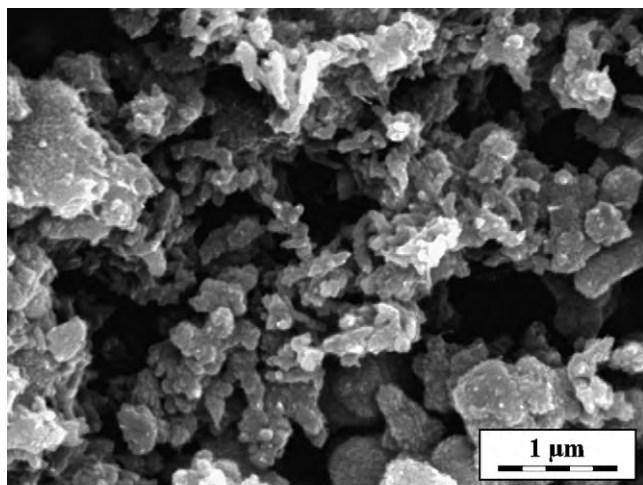
Fig. 4. The morphology of PANI prepared in 0.4 M acetic acid in the liquid state at –5 °C (top), and in the frozen reaction mixture at –25 °C (bottom).
