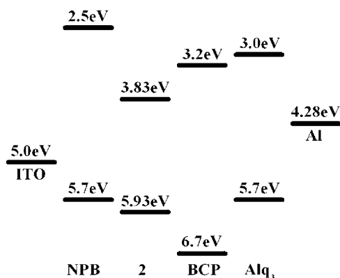
Fig. 3. Energy level diagram for the materials used in the OLED fabrication.
