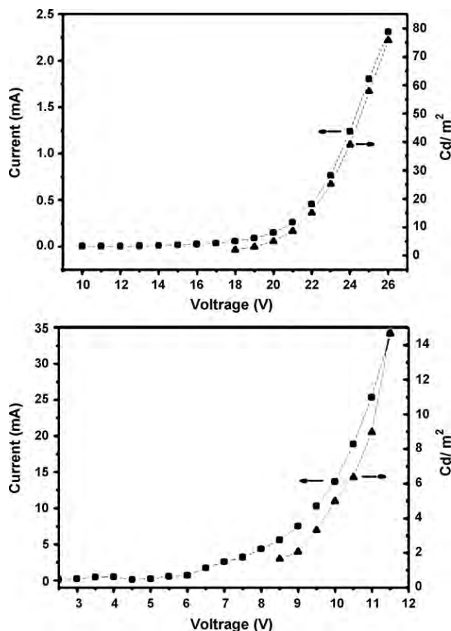
Fig. 6. Current–voltage and luminance–voltage characteristic of devices ITO/NPB/Alq 3 : 2 (1.5%)/BCP/Alq 3 /Al (up) and ITO/NPB/ 2 /Al (down).
