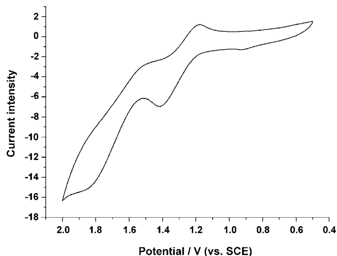
Fig. 2. Cyclic voltammogram of 2 in CHCl 3 , at a scan rate of 100 mV s -1 .
