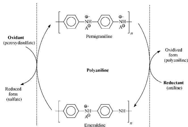
Fig. 9. The oxidant, peroxydisulfate, removes electrons from the emeraldine form of PANI, and converts it to pernigraniline. The addition of an aniline molecule to a growing PANI chain at another point results in the formation of a new constitutional unit. A transfer of electrons from the newly added aniline unit to the pernigraniline regenerates the original emeraldine form of PANI.
