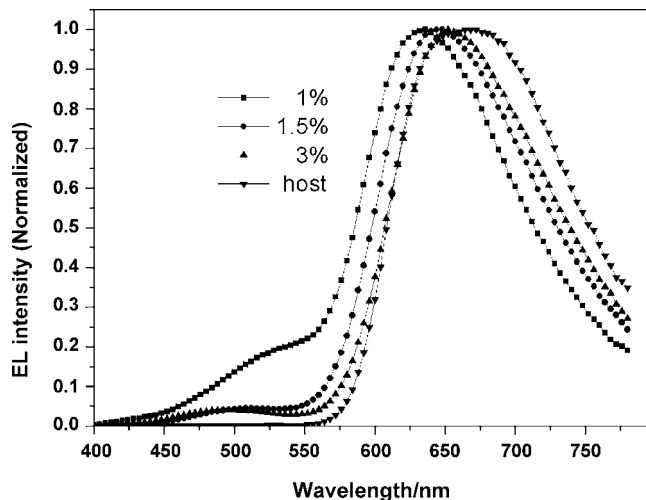
Fig. 5. EL spectra of red emitting devices with the structure ITO/NPB (60 nm)/Alq 3 : 2 (7.5 nm)/BCP (15 nm)/Alq 3 (300 nm)/Al and ITO/NPB (35 nm)/ 2 (45 nm)/Al (300 nm) (host).
