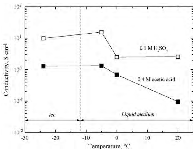
Fig. 7. The conductivity of PANI prepared at various temperatures in 0.1 M sulfuric acid (open squares) or 0.4 M acetic acid (full squares).
