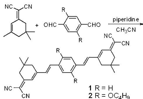
Scheme 1. Preparation of the presented DCM analogs.
