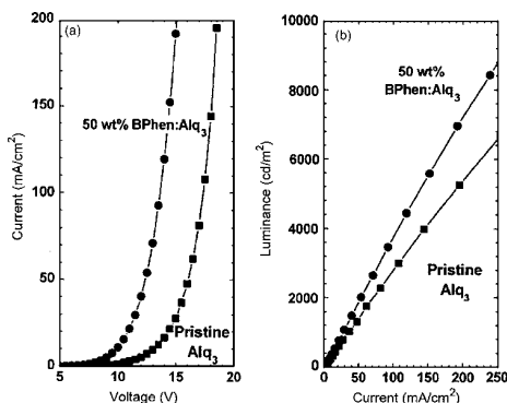
FIG. 2. Plots of (a) current-voltage and (b) luminance-current of devices without doping the EML: Device A (squares) contains a single ETL (Pristine Alq 3 ). Device C (circles) contains a cohost ET composite (50 wt % BPhen mixed Alq 3 ).
