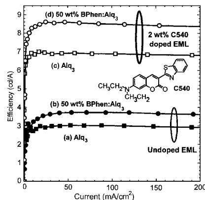
FIG. 3. Luminous efficiency of undoped EML devices—(a), (b), and C540-doped EML devices—(c), (d). The ETLs of (a), (c) and (b), (d) consist of a pristine Alq 3 layer and a 50 wt % BPhen:Alq 3 cohost layer, respectively. Inset: Molecular structure of C540.
