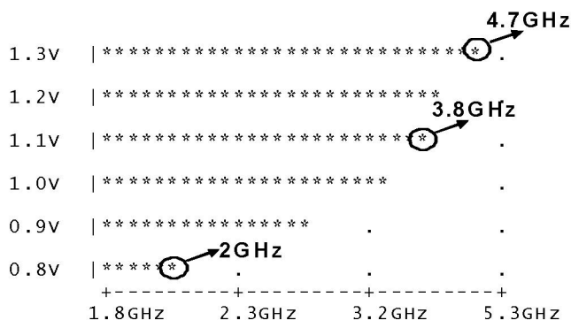
Fig. 17 Voltage-Frequency shmoo for 153Mb SRAM
