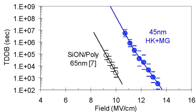
Fig. 13 NMOS TDDB time to fail vs. electric field
