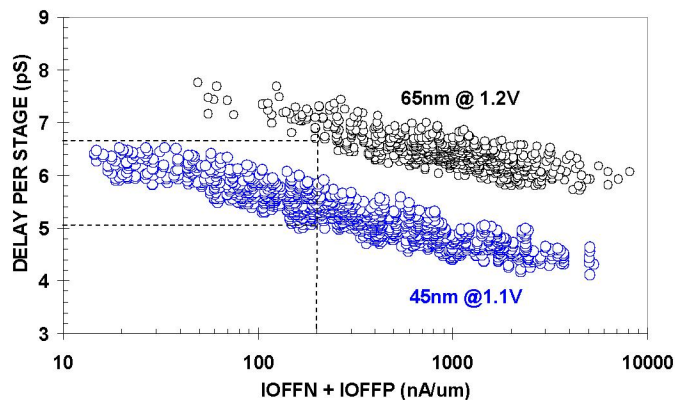
Fig.12 FO=2 ring oscillator delay vs leakage for 45nm vs 65nm
