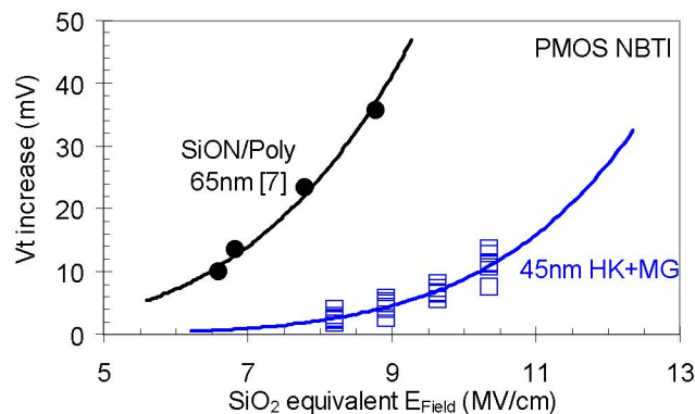
Fig. 14 PMOS NBTI V_T shift vs. electric field
